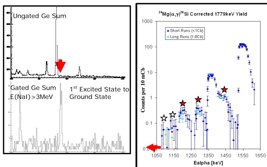
Figure 2: Preliminary results for the ^{24}\text{Mg}(\alpha,\gamma)^{28}\text{Si} reaction. The right hand panel shows the measured excitation function; new resonances are marked with a star. The left hand panel shows the relevant part of the Ge spectrum measured at the lowest observed resonance; on top the ungated spectrum, at the bottom gated on high energy \gamma -rays observed with the NaI detectors.
