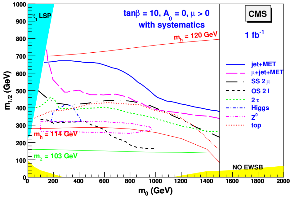
Figure 6: CMS discovery contours in various final states with leptons for an integrated luminosity of 1 \text{ fb}^{-1} .
