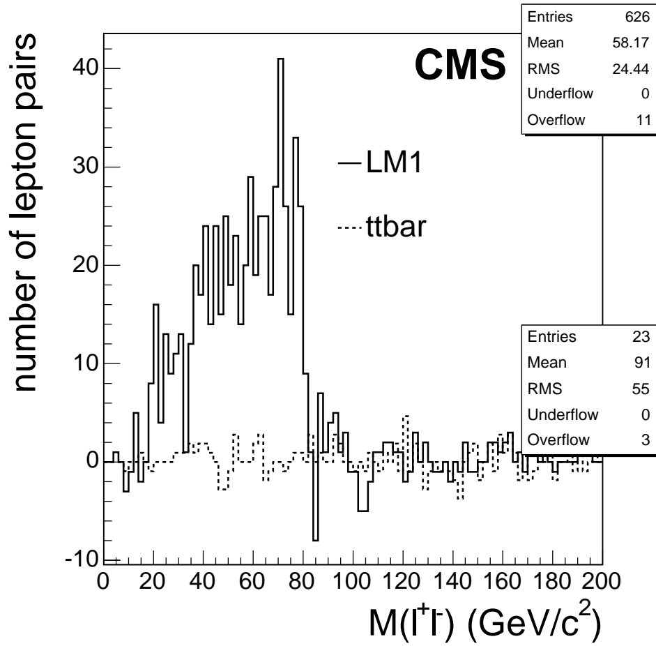
Figure 3: CMS: invariant mass distribution of same flavour opposite sign lepton pairs after the subtraction of the different flavour opposite sign lepton pair contribution. SUSY signal and t\bar{t} contribution are shown.
