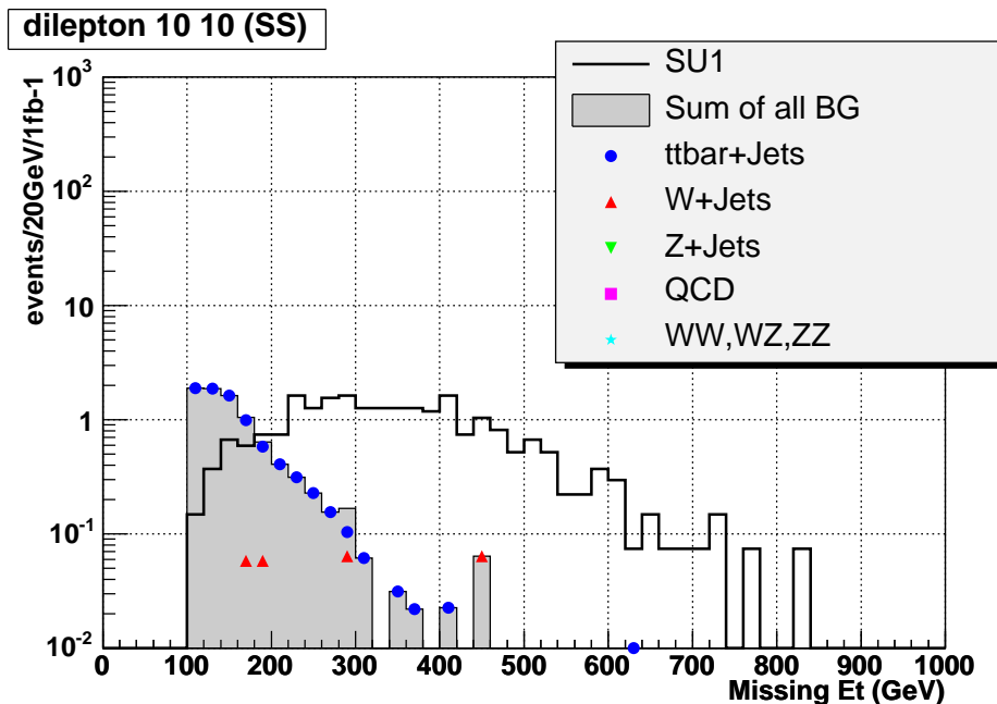
Figure 2: ATLAS: missing transverse energy distribution for events selected requiring two same sign leptons.
