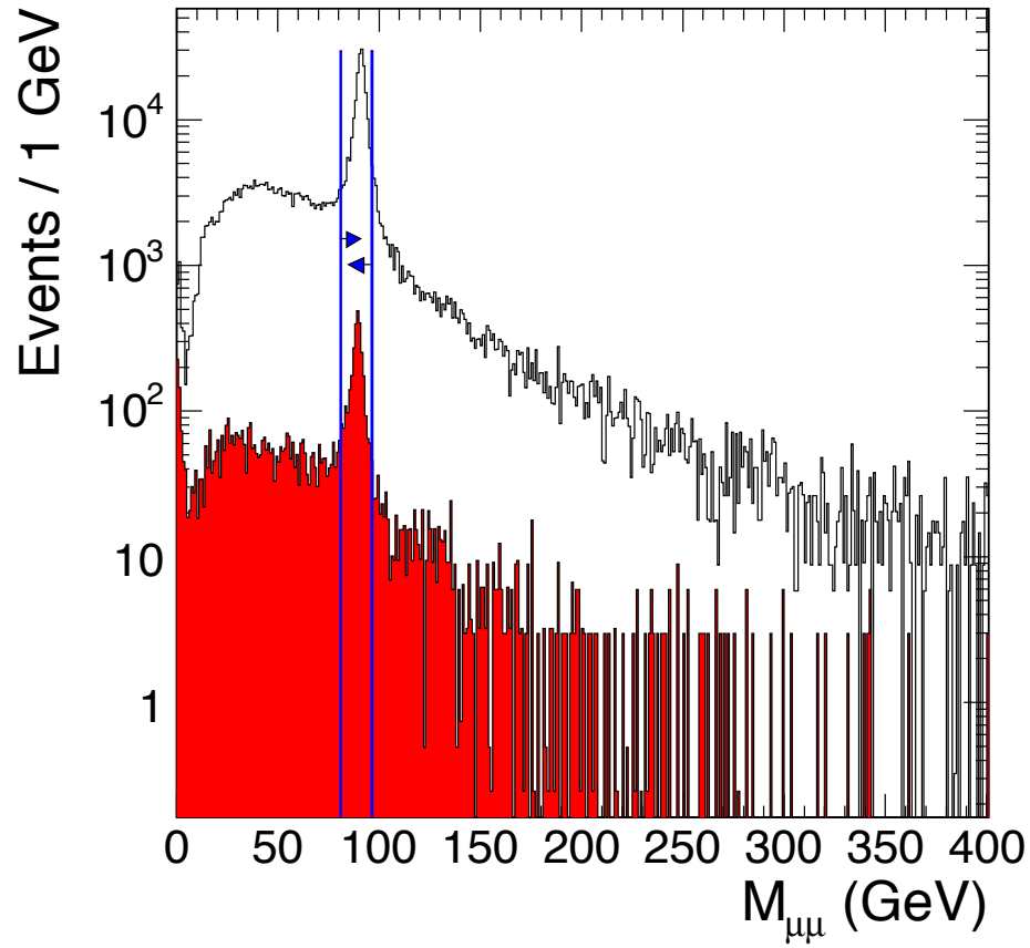
Figure 4: CMS: dilepton invariant mass distribution for supersymmetric and Standard Model events for the analysis searching Z bosons produced by supersymmetric decay chains.
