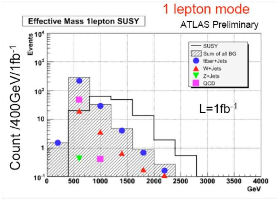
Figure 1: ATLAS: effective mass distribution after lepton and jet cuts are applied for the single lepton final state analysis
