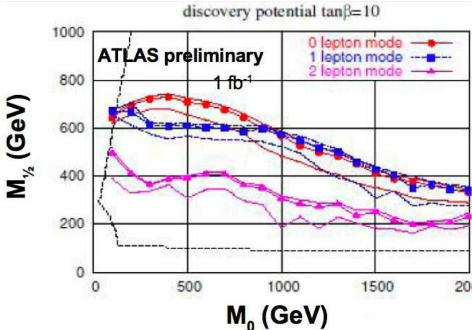
Figure 5: ATLAS discovery contours in final states with no leptons, one lepton and two leptons for an integrated luminosity of 1 \text{ fb}^{-1} .
