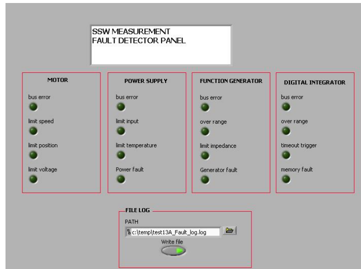
Figure 4. - Graphical interface of fault detector for rotating coil demo.
