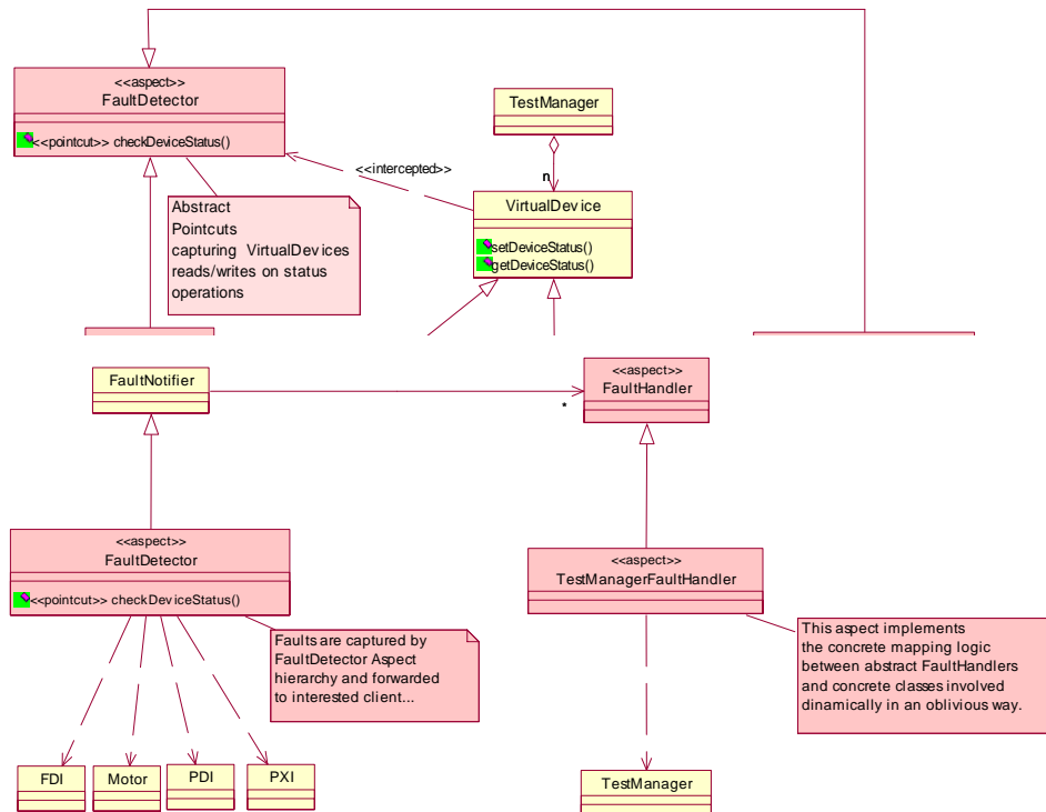
Figure 3 - Aspect mapping layer of the fault notification.
