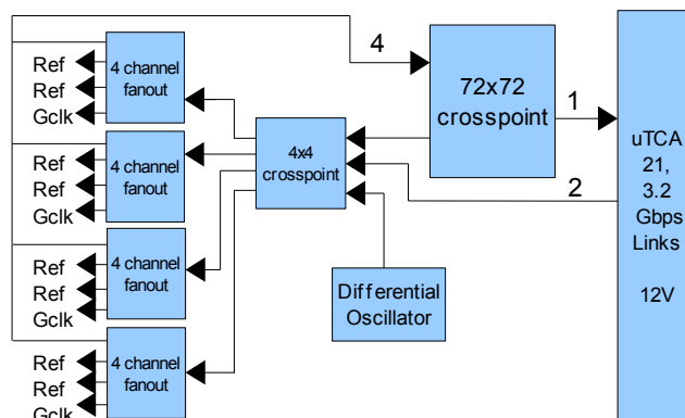
Figure 3: Module Clock tree
