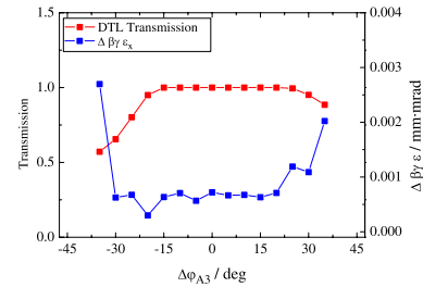
Figure 4: DYNAMION simulation of the transmission and emittance growth for different rf phases of tank A3.
