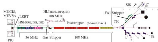
Figure 1: Schematic overview of the GSI UNILAC.
