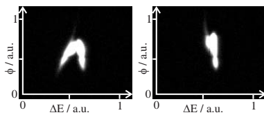
Figure 6: Longitudinal phase space distribution with Alvarez bunchers off (left) and on (right); the 1 st buncher is longitudinally focusing while the 2 nd is defocusing.
