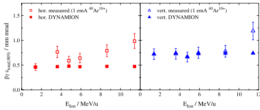
Figure 3: Measured and calculated (DYNAMION) transverse beam emittances for different Alvarez energies (3.6, 4.8, 5.9, 8.6 and 11.4 MeV/u). The emittance at injection is measured ahead the Alvarez at 1.4 MeV/u.
