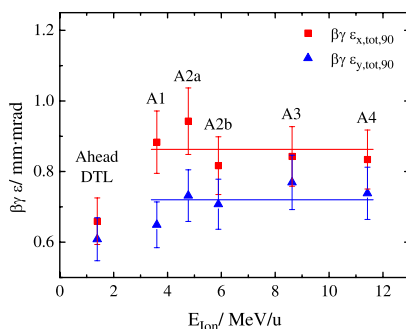
Figure 7: Normalised transverse emittances at different beam energies.
