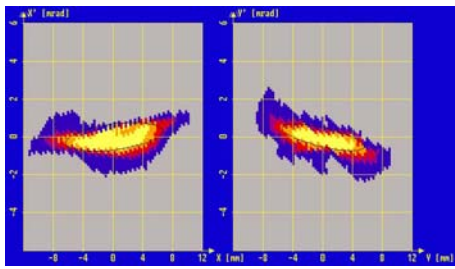
Figure 5: Measured transverse beam emittances for optimised UNILAC settings at 11.4 MeV/u and p_{\text{stripper}} = 2000 mbar.
