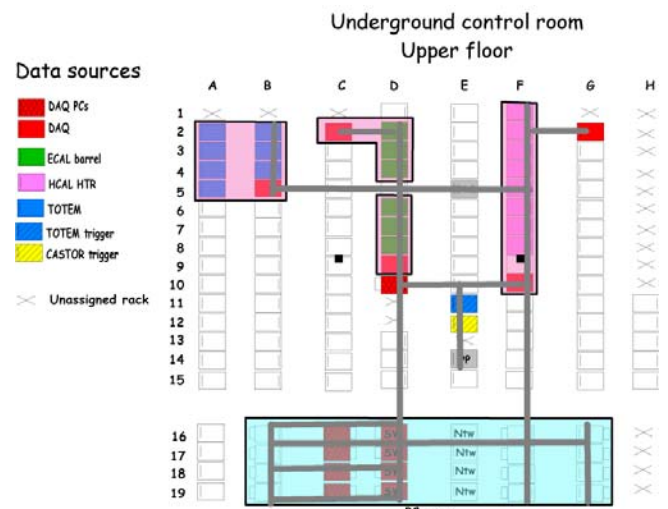
Figure 2: DAQ rack location and cable trays in USC55
