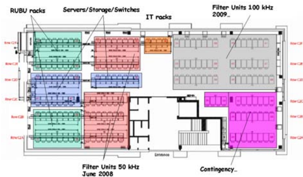
Figure 6: Rack layout in CMS computer room
