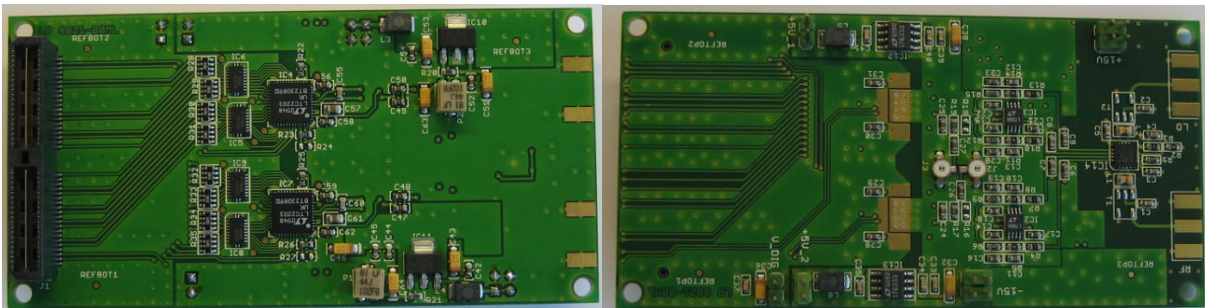
Fig. 1: Top and bottom view of the iq-detector
