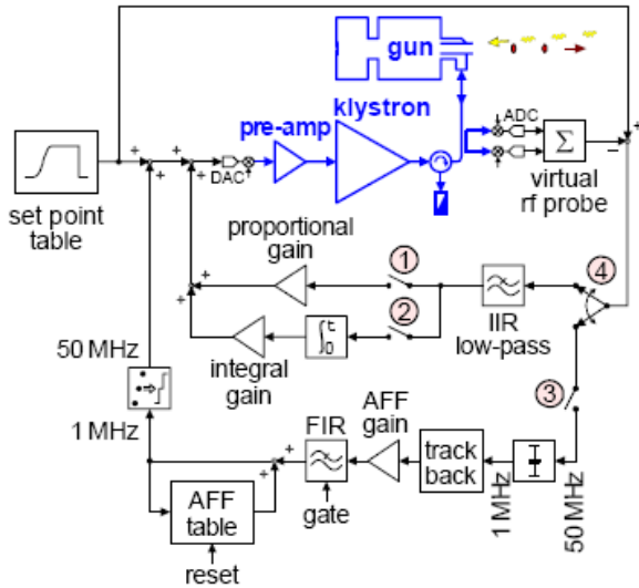
Figure 1: Block diagram of the gun rf control implemented in SimCon (black) surrounding the high power rf (blue). DACs in front of the vector modulator ( \otimes ) and ADCs after down converters ( \otimes ) are part of SimCon.
