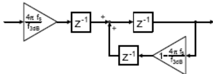
Figure 2: Recursive low-pass with infinite impulse response. The filter gain values depend on the processing frequency f_s = 50 MHz and the filter frequency f_{3dB} .
