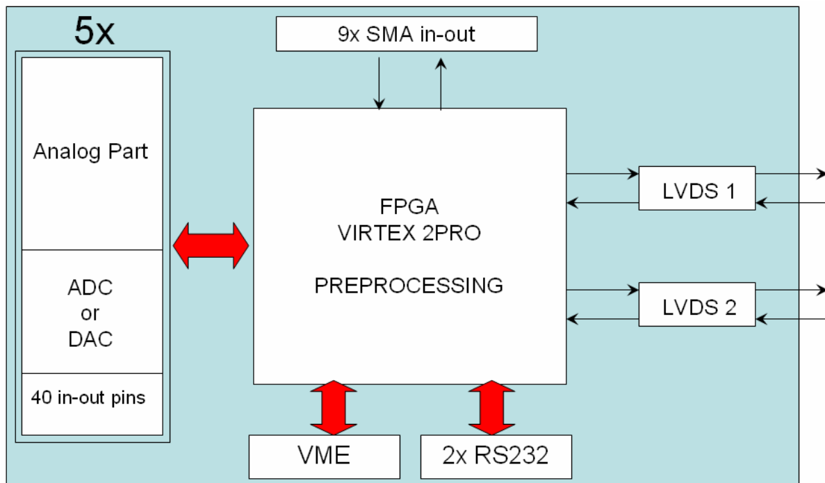
Fig.3: Block diagram of the motherboard
