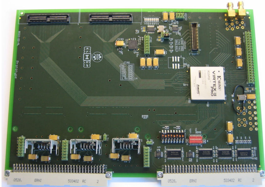
Fig. 2: Top view of the motherboard (bottom layer has 3 additional connectors)
