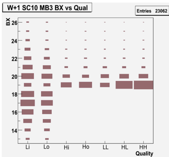
Figure 11: Bunch crossing number versus quality of the trigger primitives.
