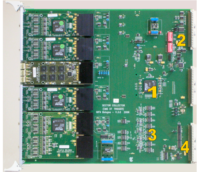
Figure 4: The Trigger Sector Collector board.
