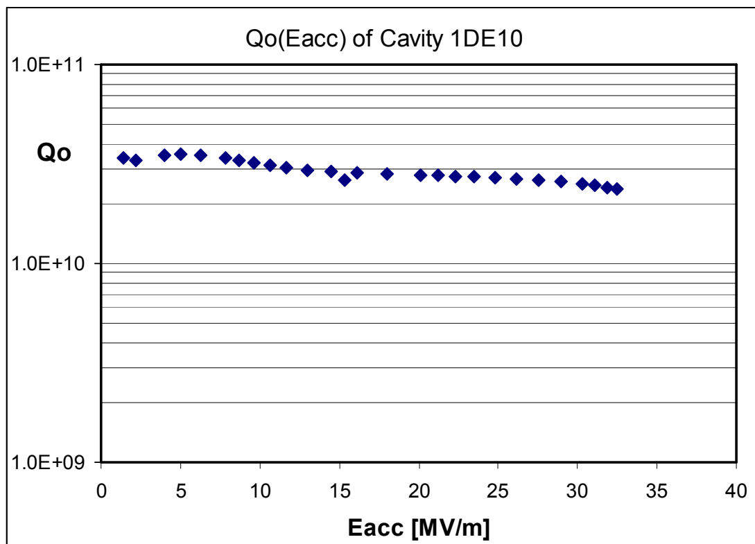
Figure 7: Recent best Q_0(E_{acc}) -performance after dry-ice cleaning with new capillary
