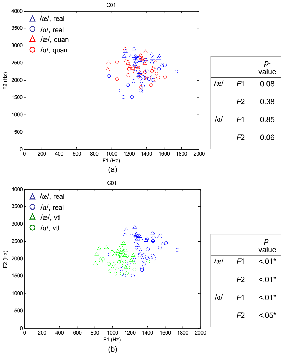
Figure 4.23. F1-F2 plots and p -values from real data at Time 2 for the subject C01 and from the predictions for them. (a) the real data vs. predictions based on quantal relations (b) the real data vs. predictions based on vocal tract growth.
