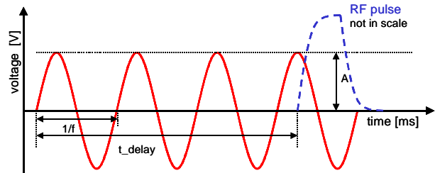
Figure 2. Shape of the pulse applied to piezoelement. Parameters which can be set in the system are marked
