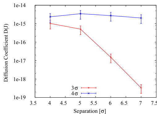
Figure 4: Diffusion coefficients (from BBSIM) vs beam separation at initial amplitudes of 3 and 4 \sigma . Tunes at (0.68, 0.69).
