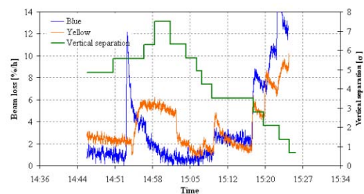
Figure 2: Beam loss and vertical separation at 100 GeV. Before 15:00h the Blue beam was moved to change the separation, after 15:00h the Yellow beam was moved.
