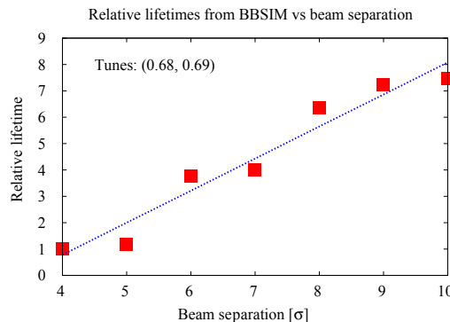
Figure 5: Relative lifetime vs separation with BBSIM.
