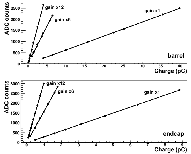
Figure 3: VFE outputs in ADC counts versus injected charge for the barrel (top figure) and endcap VFE (bottom figure) representing calibration curves for the three gains 1, 6, and 12.
