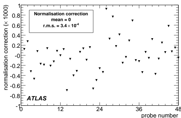
Figure 7. Probe normalisation corrections for the high field maps.
