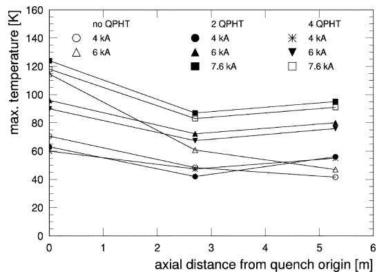
Fig. 7. Temperature evolution as function of the axial distance from the quench origin, for different currents and with no, 2 or 4 QPHTs. Quench origin is at the point 109 heater.
