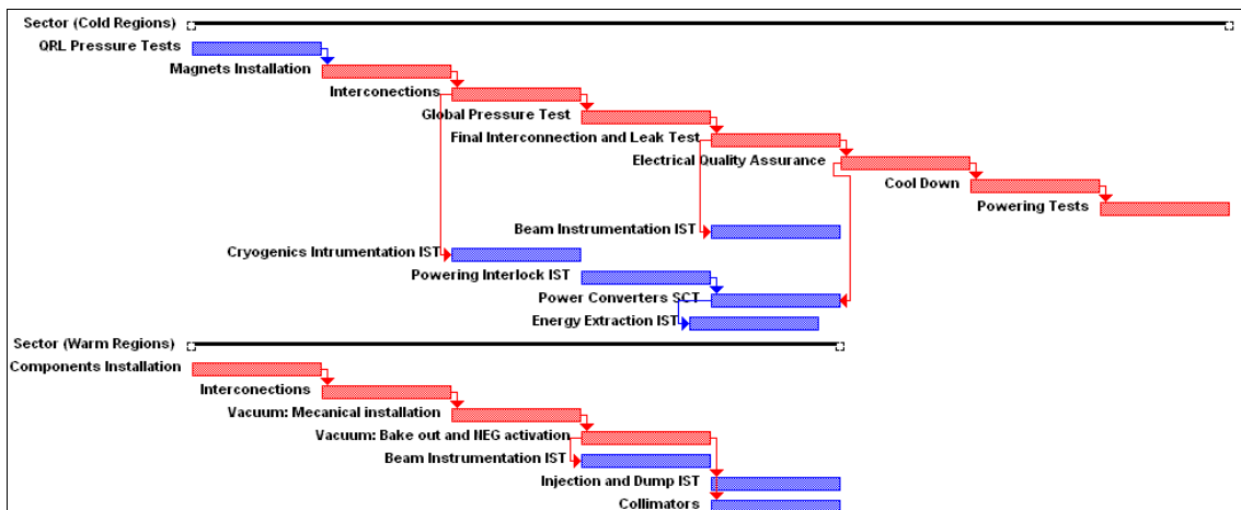
Figure 2: IST dependencies with the activities on the critical path and in between ISTs. Red bars correspond to installation activities and blue bars to IST (bar lengths do not represent the precise duration of the activities)
