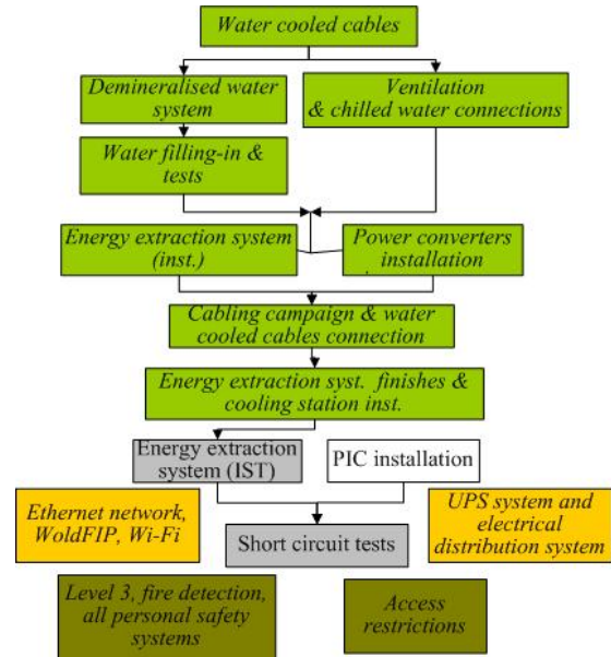
Figure 1: Requirements of the short circuit test:
