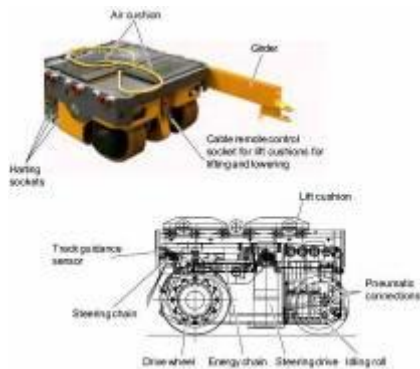
Figure 2: Warm magnet transport vehicle buggy
