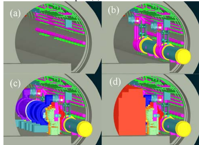
Figure 2: Phases of the LHC Machine Installation.
