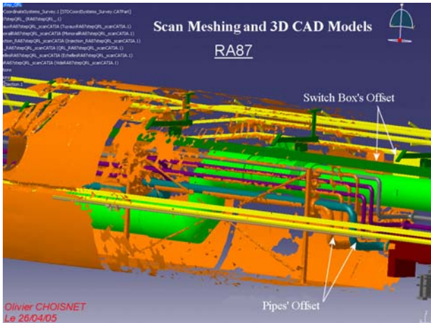
Figure 6: Meshing and 3D models superimposed in the CATIA CAD tool.
