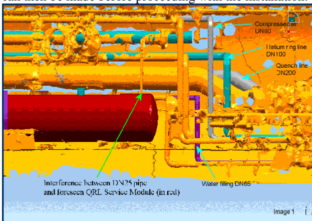
Figure 7: Interference identification.
