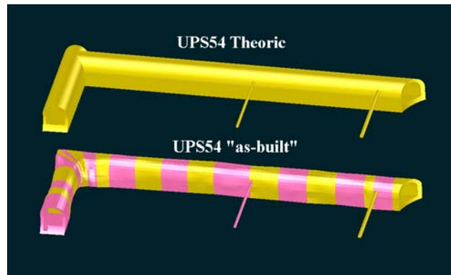
Figure 8: Tunnel as-built model from scanned points.
