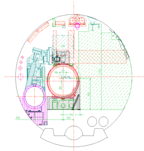
Figure 1: Typical Section of the LHC Tunnel.
