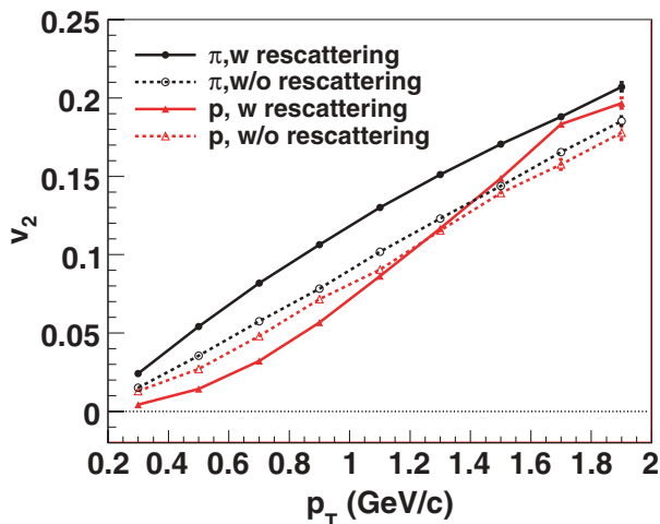
FIG. 5. (Color online) Transverse-momentum dependence of the elliptic flow parameter for pions and protons. Solid (dashed) lines are with (without) hadronic rescattering.
