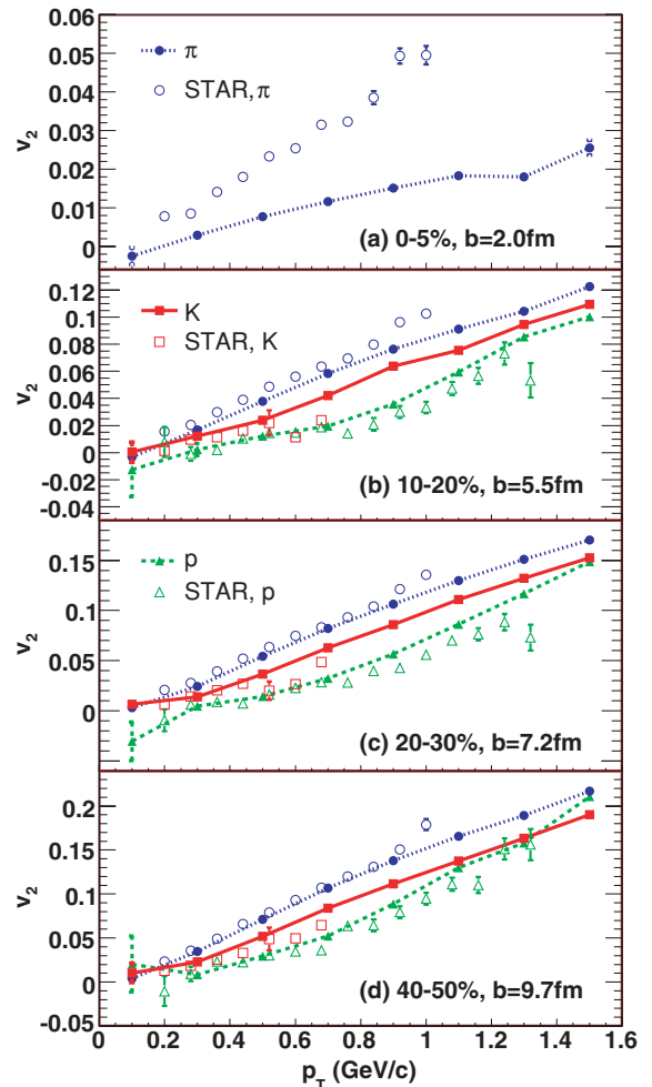
FIG. 4. (Color online) Transverse-momentum dependence of the elliptic flow coefficient v_2 for pions (dotted blue), kaons (solid red), and protons (dashed green) from the hybrid model, compared with STAR data for v_2\{2\} from 200A GeV Au+Au collisions, in four centrality classes [52].
