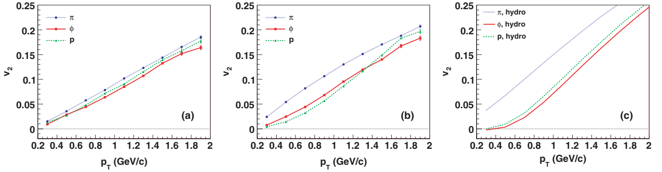
FIG. 9. (Color online) Transverse-momentum dependence of the elliptic flow parameters for pions (dotted blue), protons (dashed green), and \phi mesons (solid red), for Au+Au collisions at b = 7.2 fm. (a) Before hadronic rescattering. (b) After hadronic rescattering. (c) Ideal hydrodynamics with T_{\text{th}} = 100 MeV. The results for pions and protons are the same as shown in Fig. 5.
