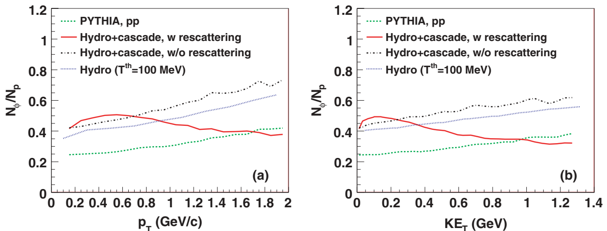
FIG. 8. (Color online) The \phi/p ratio as a function of p_T (left panel) and of transverse kinetic energy \text{KE}_T \equiv m_T - m_0 (right panel) for different scenarios: central Au+Au collisions in the hybrid model, without hadronic rescattering, and in the hydrodynamic model with T_{\text{th}} = 100 MeV (dotted). The corresponding ratio for proton-proton collisions (extracted from the PYTHIA fit to the experimental data shown in Fig. 10 below) is shown for comparison as the dashed line. See text for more discussion.
