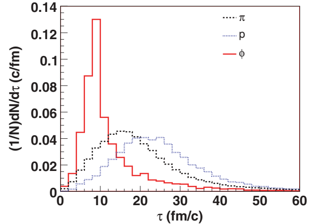
FIG. 6. (Color online) Normalized distribution of freeze-out times for pions (dashed), protons (dotted), and \phi mesons (solid) for |y| < 1 in Au+Au collisions at b = 2.0 fm.
