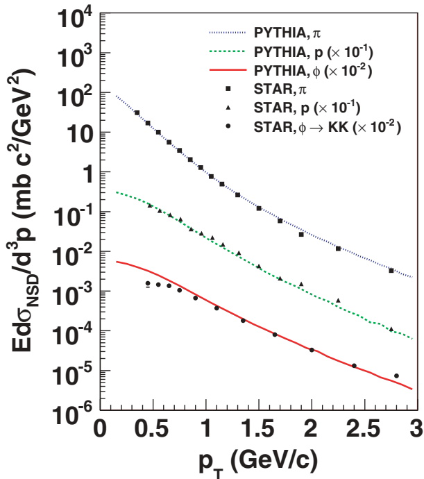
FIG. 10. (Color online) Invariant cross sections as a function of p_T in nonsingly diffractive pp collisions for pions, protons, [72] and \phi mesons. Dotted, dashed, and solid lines are results from PYTHIA for pions, protons, and \phi mesons, respectively.
