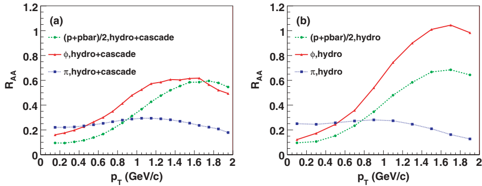
FIG. 11. (Color online) Nuclear modification factors R_{AA} for pions (blue), \phi mesons (red), and protons/antiprotons (green) for Au+Au collisions at b = 3.2 fm (corresponding to 0–10% centrality). Shown are predictions from (a) the hybrid model and (b) from ideal hydrodynamics with T_{th} = 100 MeV.
