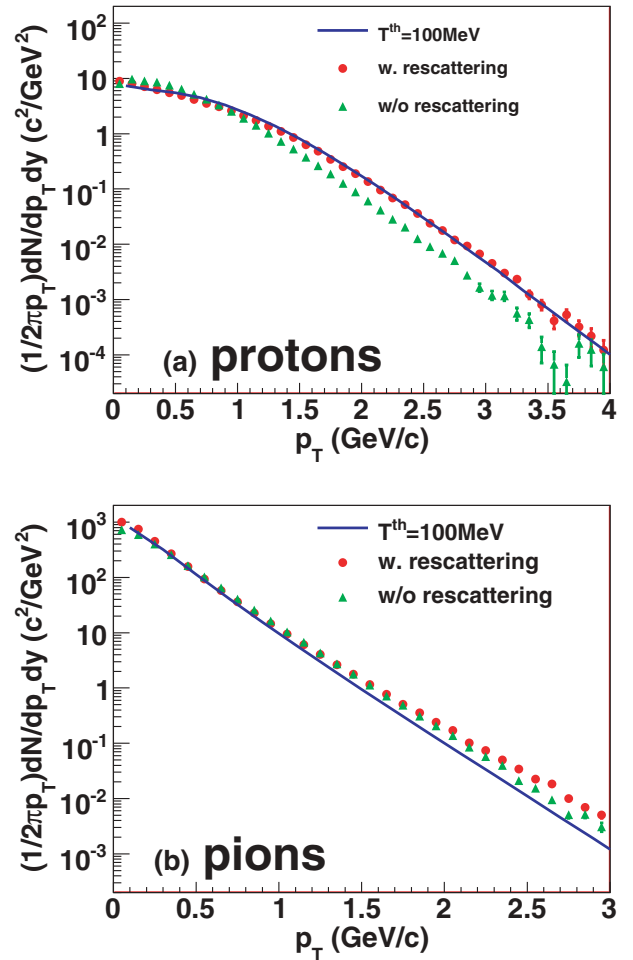
FIG. 1. (Color online) p_T spectra with and without hadronic rescattering for (a) protons and (b) pions at midrapidity for Au+Au collisions at b = 2 fm, compared with results from ideal hydrodynamics decoupling at T_{\text{th}} = 100 MeV.
