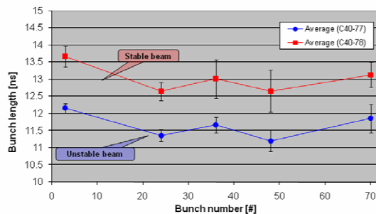
Figure 6: Bunch length difference for the two 40 MHz cavities at 100 KV, before calibration (80 MHz at 0 KV).
