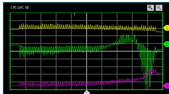
Figure 3: PS to SPS transfer line BPM signals, sum (1), horizontal delta (2) and vertical delta (3).
