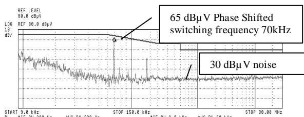
Fig. 9: Differential mode output voltage noise.
