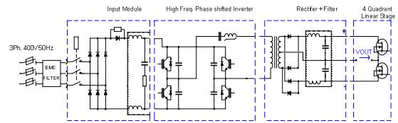
Fig. 3: Voltage Source Power Converter topology.
