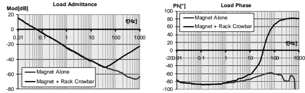
Fig. 10: Output load transfer function.
