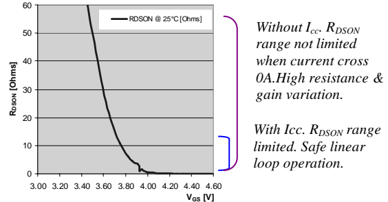
Fig. 5: MOSFET R DS(on) gain vs V GS .
