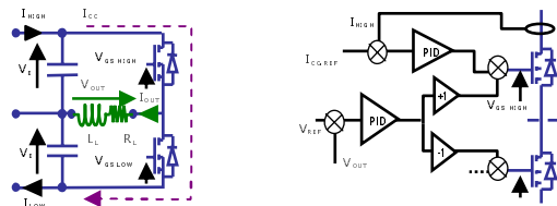
Fig. 4: Circulating Current Principle.
