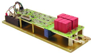
Fig. 7: LHC120A-10V Crowbar.
