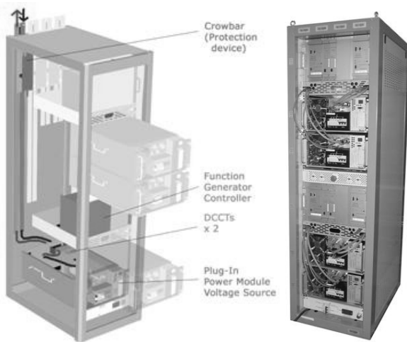
Fig. 2: LHC120A-10V Rack.
