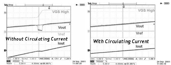
Fig. 6: Circulating current effect.
