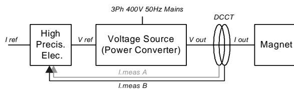
Fig. 1: LHC Power Converter.
