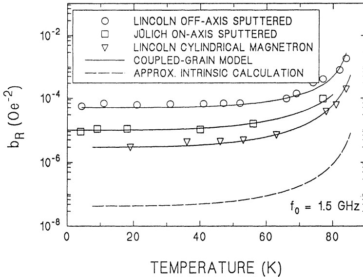
FIGURE 5: b_R(T) of different thin films as compared to the theoretical value.
