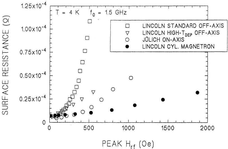
FIGURE 4: R_s vs H_{rf} of different thin films.
