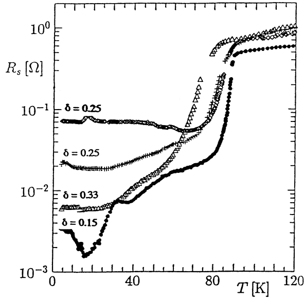
FIGURE 3: R_s(T) as a function of oxygen content and order ( \bullet : as prepared, \diamond : 1 h, 500 °C, 1 bar O_2 , quench cooled, + : 0.5 h, 250 °C, 1 bar O_2 , slowly cooled, \Delta : 1 h, 500 °C, 0.15 bar O_2 , slowly cooled).
