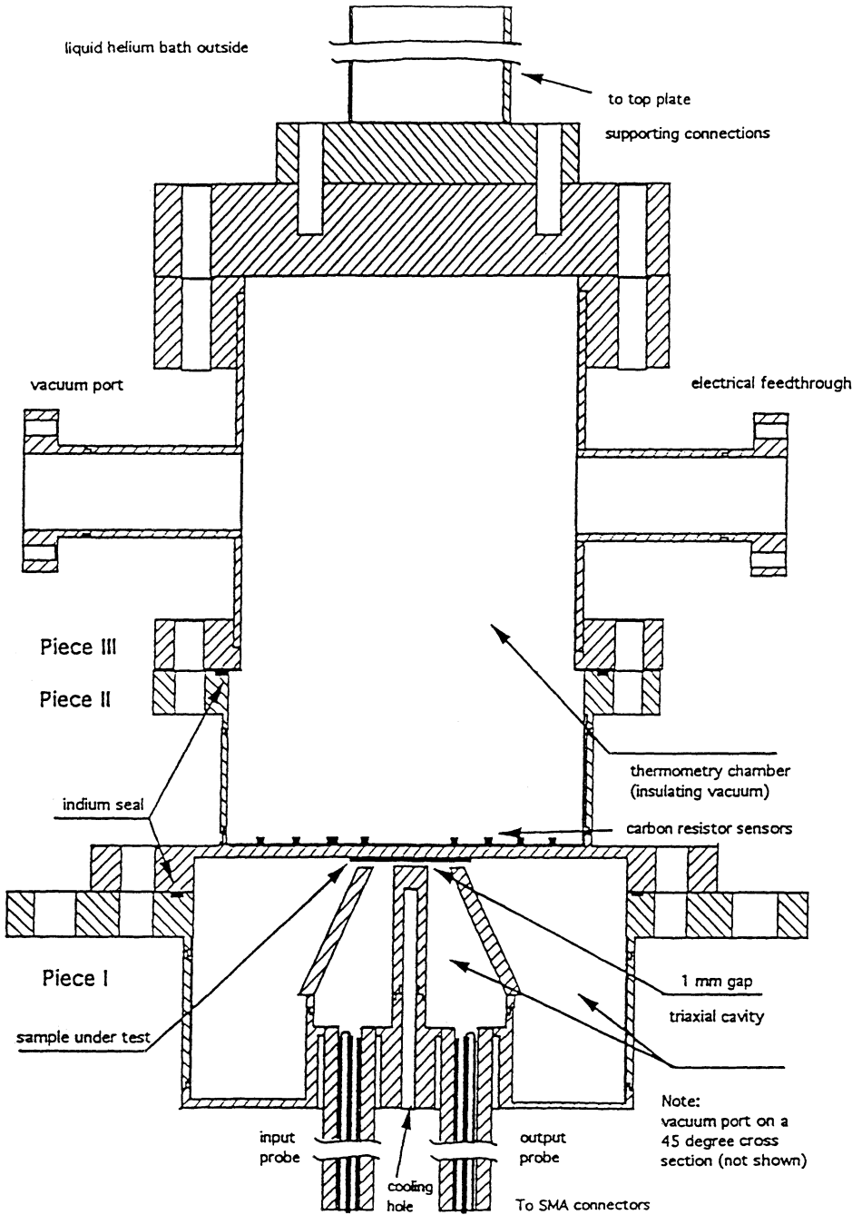
FIGURE 1: Configuration of the niobium triaxial cavity.
