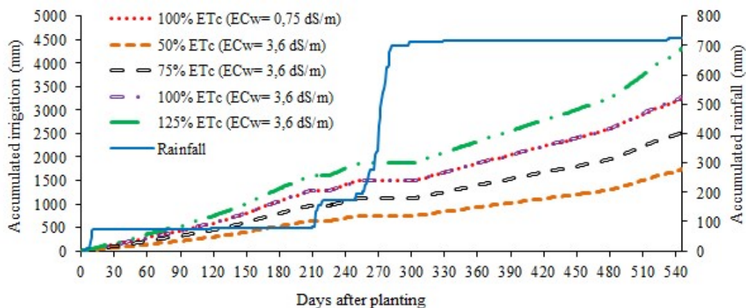
Figure 2. Accumulate irrigation applied to different treatments and accumulated rainfall during the experimental period.
