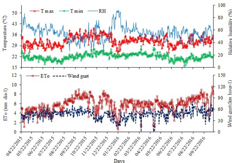
Figure 1. Maximum and minimum temperatures (Tmax and Tmin, respectively), relative humidity (RH), and gusts of wind, rainfall, and reference evapotranspiration (ET 0 ) during the conduction of the experiment.
