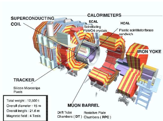
Fig. 18.1: Schematic view of the CMS detector
