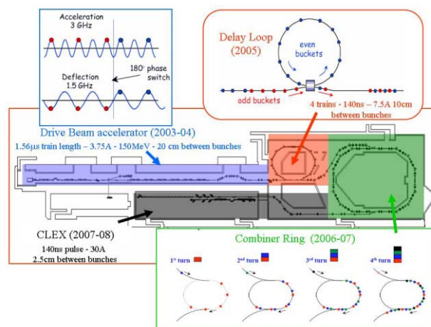
Figure 2: Overview of the CTF3 complex
