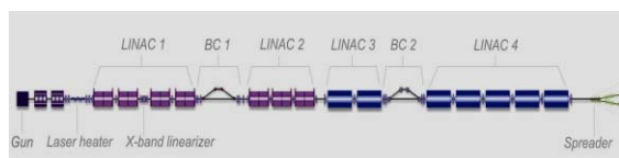
Figure 1: Overview of FERMI at ELETTRA
