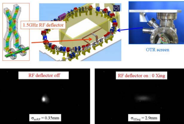
Figure 3: RF deflector measurement at CTF3
