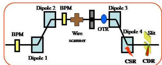
Figure 4: Magnetic chicane monitors at FERMI
