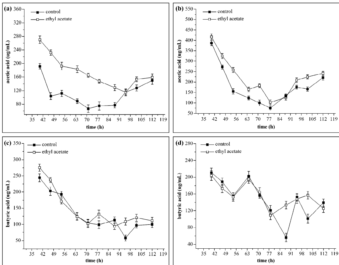
Figure 4. Time course analyses of intracellular organic acid (a, c) and extracellular organic acid (b, d) levels with and without the addition of ethyl acetate in a 15-L fermentor. Ethyl acetate (□) and control (■).
