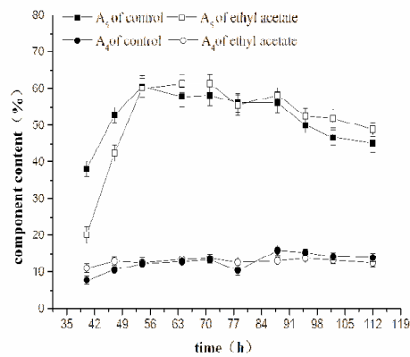
Figure 3. Time course analysis of components upon addition of ethyl acetate in a 15-L fermentor. Ethyl acetate (□,○) and control (■,●)
