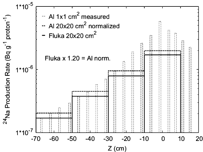
Fig. 8. ^{24}\text{Na} Production rate at different distances from the beam axis predicted on 20 \times 20 \text{ cm}^2 Al foils from MonteCarlo simulation (continuous line) compared with the one directly measured with the activation-foils technique (dotted lines).
