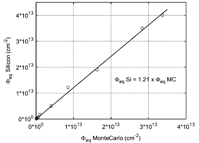
Fig. 9. Equivalent fluence from Silicon detectors, plotted versus the equivalent fluence calculated from Monte Carlo simulations.
