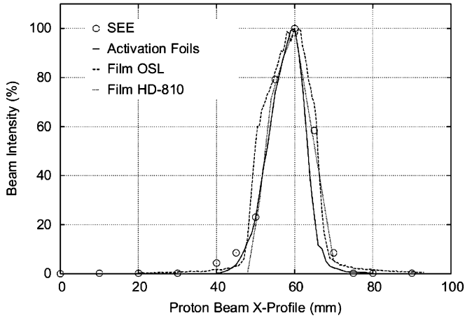
Fig. 6. BPM measurements (circle marks) compared with the profiles obtained by means of OSL, activation foils and Gafchromic films (different continuous lines)
