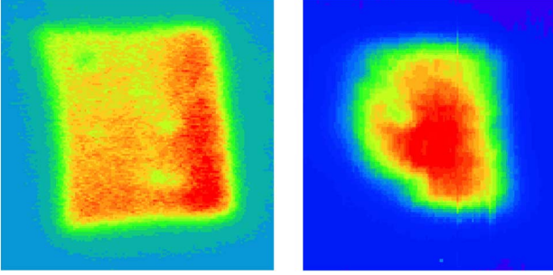
Fig. 5. High-resolution beam profiles measured by a 100 \mu\text{m} OSL film. Big beam-spot of about 4.5 \times 4.5 \text{ cm}^2 (left hand side) and standard beam spot of about 2 \times 2 \text{ cm}^2 (right hand side) (Color version available online at http://iee-explore.ieee.org ).
