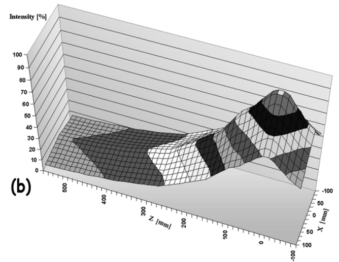
Fig. 3. Particle spectra in IRRAD2 cavity at 10 centimeters from the beam axis normalized to one impinging 23 GeV proton (a) and particle profile as measured by the Al activation method in the IRRAD2 cavity in function of the distance from the beam axis Z (b).
