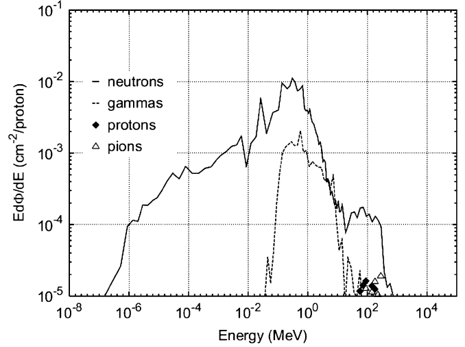
Fig. 7. Particle spectra in IRRAD2 cavity at 50 centimeters from beam axis normalized to one impinging 23 GeV proton.
