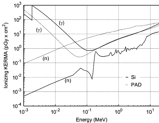
Fig. 11. Neutron (n) and photons ( \gamma ) KERMA values in Si and PAD in the energy range from 1-keV to 20-MeV.
