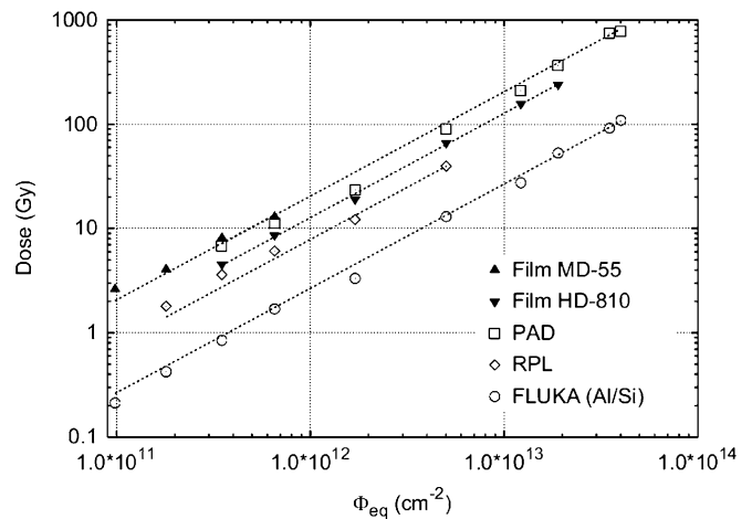
Fig. 10. Comparison among the different TID measured at 50 cm from the beam axis obtained by different dosimetric means. The dotted lines have been plotted as guidelines within different data sets.
