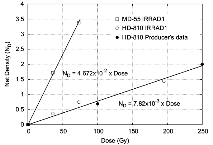
Fig. 4. Gafchromic dosimetric films HD-810 and MD-55. Calibration curves obtained in IRRAD1 facility compared with producer data.
