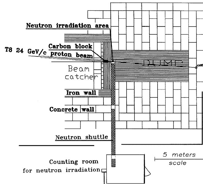
Fig. 2. Layout of the IRRAD2 irradiation Facility.
