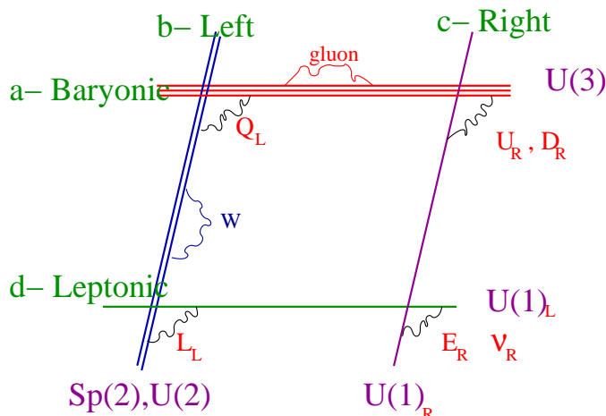
Figure 1: Quarks and leptons at intersecting branes.
