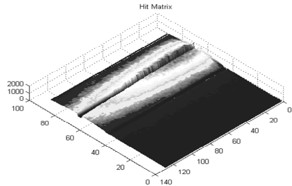
Figure 9: Hit map detail between two FPIX2.1 chips
