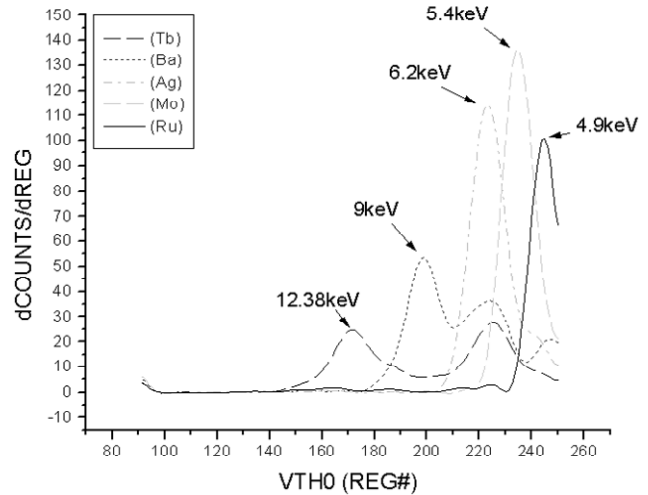
Figure 8: Test results of a pixel sensor using radioactive sources
