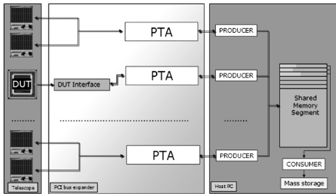
Figure 11: Functional diagram of the test beam DAQ
