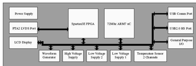
Figure 5: Functional diagram of the FEM
