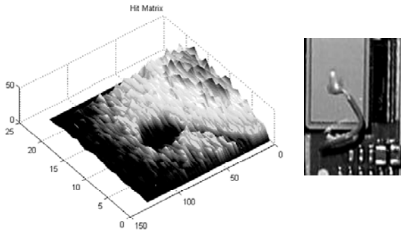
Figure 10: Hit map footprint of bias connection
