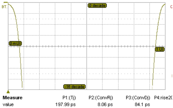
Figure 5: Bathtub curve.
