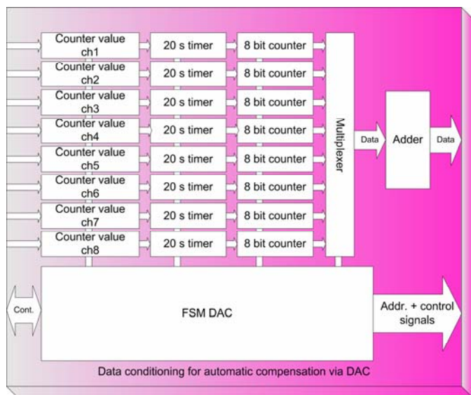
Figure 6: Block diagram DAC interface
