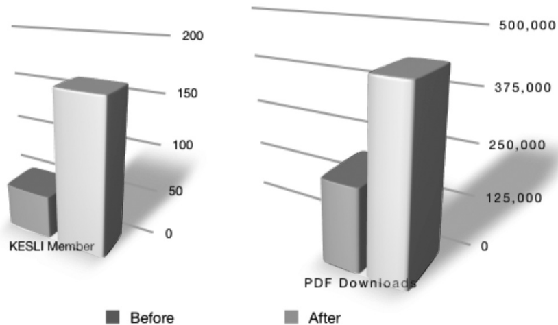
Fig. 5. Analysis Result
