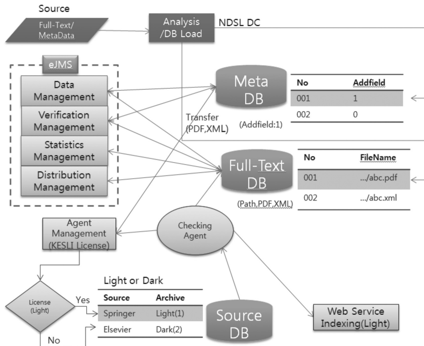
Fig 1. System Process
