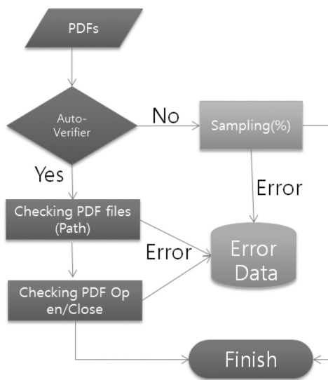
Fig. 2. Verifier Process
