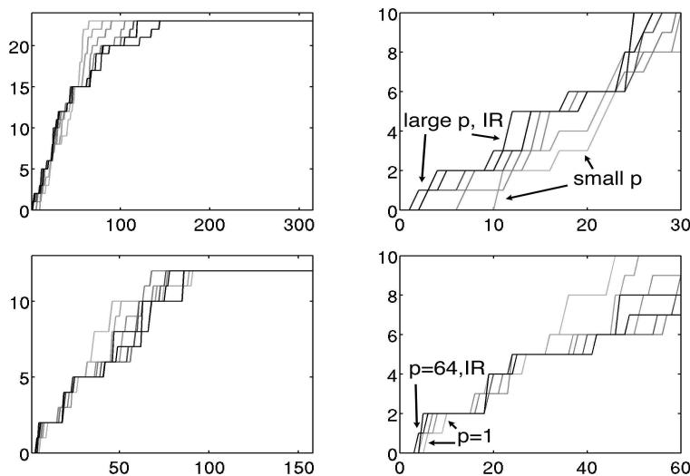
Figure 7: ROC Curves for the P-Norm Push and IR Push on the housing data set. All plots are number of true positives vs. number of false positives. Upper Left : Full ROC Curves for training. Upper Right : Zoomed-in version of training ROC Curves. Lower Left : Full ROC Curves for testing. Lower Right : Zoomed-in version of testing ROC Curves.
