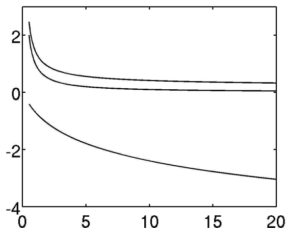
Figure 3: Discounting factor for discounted cumulative gain 1/\ln(1+z) (upper curve), discounting factor for the average of the reciprocal of the ranks 1/z (middle curve), and new discounting factor -\ln(1+z) (lower curve) versus z .
