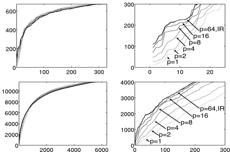
Figure 5: ROC Curves for the P-Norm Push and IR Push on the MAGIC data set. All plots are number of true positives vs. number of false positives. Upper Left : Full ROC Curves for training. Upper Right : Zoomed-in version of training ROC Curves. Lower Left : Full ROC Curves for testing. Lower Right : Zoomed-in version of testing ROC Curves.
