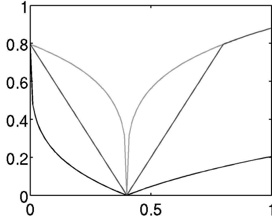
Figure 8: Functions |a^{1/p} - b^{1/p}| (lower curve), |a - b|^{1/p} (upper curve), and \min(|a - b|a^{(1/p)-1}, |a - b|^{1/p}) (middle curve) versus b . For this figure p = 4 and a = 0.4 . One can see that in most cases, |a - b|a^{(1/p)-1} is a better approximation to |a^{1/p} - b^{1/p}| than |a - b|^{1/p} .
