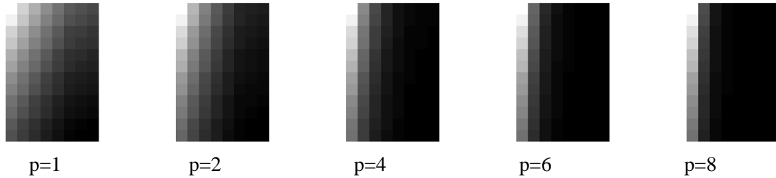
Figure 1: Contribution of each positive-negative pair to the objective R_{p,\text{exp}} . Each square represents an i, k pair, where i is an index along the vertical axis, and k is along the horizontal axis. Lighter colors indicate larger contributions to R_{p,\text{exp}} . The upper left corner represents the highest (worst) ranked negative and the lowest (worst) ranked positive.
