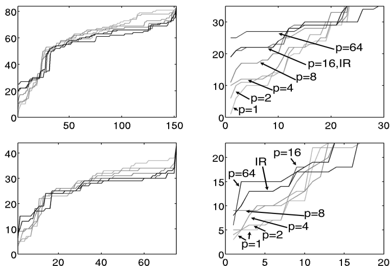
Figure 6: ROC Curves for the P-Norm Push and IR Push on ionosphere data set. All plots are number of true positives vs. number of false positives. Upper Left : Full ROC Curves for training. Upper Right : Zoomed-in version of training ROC Curves. Lower Left : Full ROC Curves for testing. Lower Right : Zoomed-in version of testing ROC Curves.
