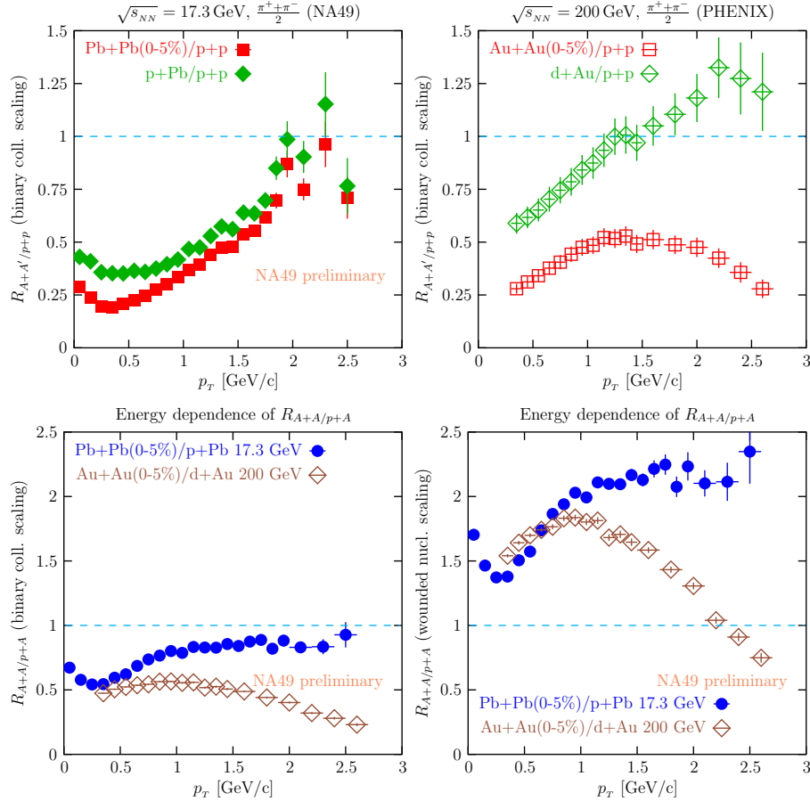
Fig. 3. Upper panels: energy dependence of the nuclear modification factor R_{A+A'}/p+p for \pi^\pm from top ion-SPS to top RHIC energies. Lower left panel: energy dependence of the nuclear modification factor R_{A+A}/p+A for \pi^\pm from top ion-SPS to top RHIC energies (binary collision scaling). Lower right panel: the same with wounded nucleon scaling.
