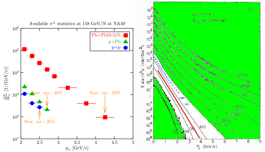
Fig. 2. Left panel: currently available p_T range for \pi^\pm in p+p, p+Pb and Pb+Pb collisions at 158 GeV/nucleon at midrapidity in the experiment NA49. The p+p and p+Pb range is severely limited by statistics. Right panel: a compilation of all existing data for \pi^- production in the p+p collisions in the nearby energy range, shown together with the new NA49 data. As can be seen there are no data near 158 GeV, and the shape of the spectra changes rapidly with beam energy from convex to concave (transition shown by the solid line).
