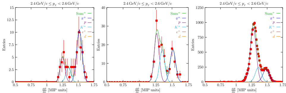
Fig. 1. Demonstration of the reliability of the inclusive particle identification by specific energy loss at high p_T , in p+p, p+Pb and Pb+Pb(0-5%) collisions, respectively.
