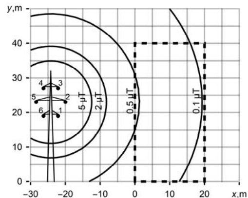
Fig. 6. Distribution of double-circuit OHL magnetic field when \varphi_1=\varphi_4 , \varphi_3=\varphi_6
