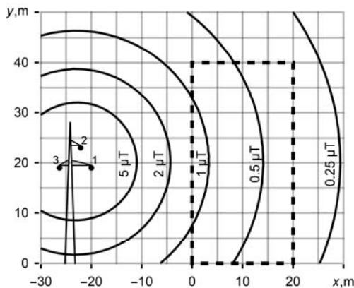
Fig. 2. Distribution of single-circuit OHL magnetic field
