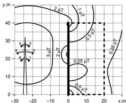
Fig. 8. Distribution of double-circuit OHL magnetic field when using plane grid shield
