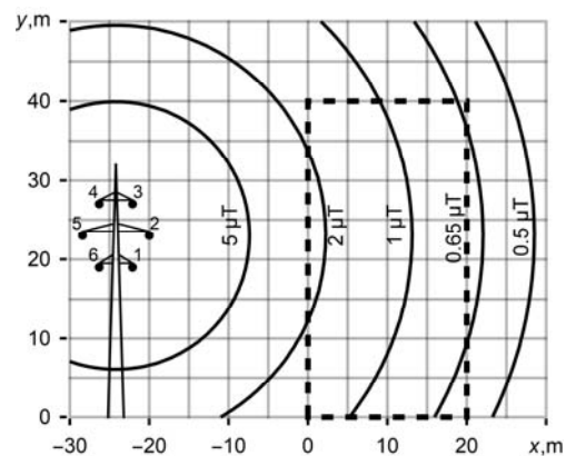
Fig. 7. Distribution of double-circuit OHL magnetic field when \varphi_1=\varphi_6 , \varphi_3=\varphi_4
