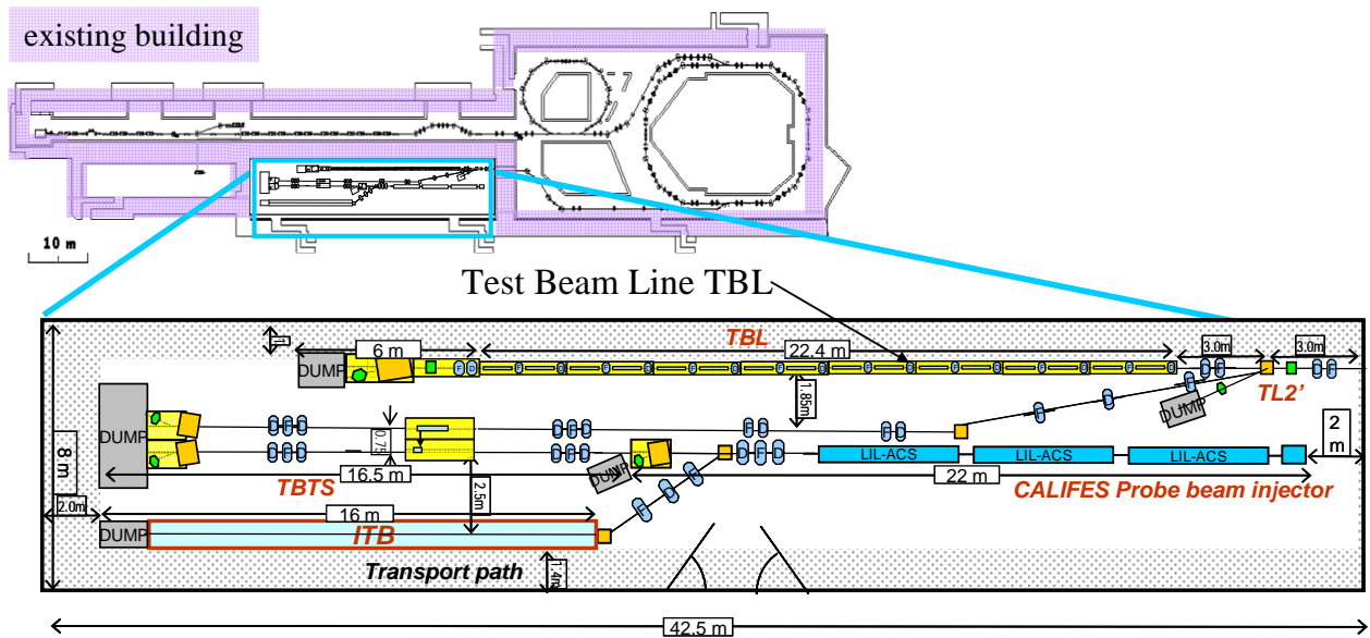
Figure 3 CLEX (=CLIC EXperimental area) of CTF3 TBL =Test Beam Line TBTS =Two Beam Test Stand ITB =Instrumentation Test Beam
