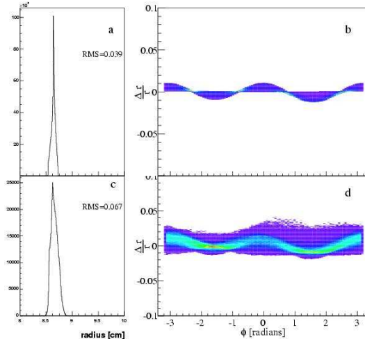
Fig. 2. Geometrical aberrations from ray tracing in the actual geometry of the detector. Panels a and b correspond to the first set of pion moving all along the axis of the detector. Panels c and d were obtained with measured tracks that have different angles of incidence as well as different entrance point locations, this set shows the strongest geometrical aberrations. For both sets of pions, the left panel shows the distribution of radii, and the right ones display the relative deviation from a perfect circle as a function of the azimuth angle.
