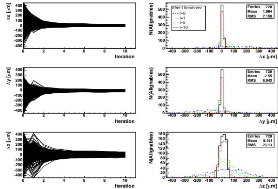
Figure 4. Alignment of the CMS Pixel detector using the HIP algorithm.
