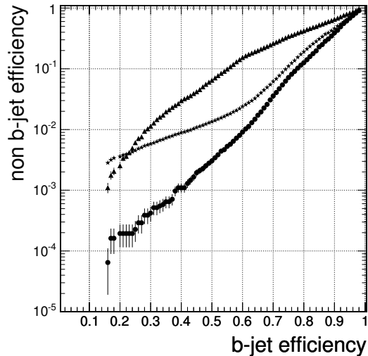
Figure 6. B-tagging performance for c (top), g (middle) and uds (bottom) jets.
