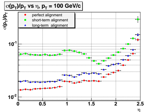
Figure 3. Transverse momentum resolution in the CMS Tracker with and without misalignment.
