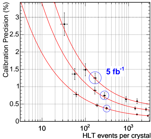
Figure 5. ECAL calibration precision.
