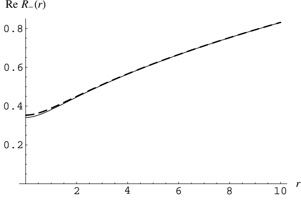
FIG. 4: Numerical results for the example (5.44) confirm the existence of Witten spinors that are regular at the origin and have the correct behavior at large r . The solid line is \text{Re } R_- = \text{Im } R_+ = \text{Re } \tilde{R}_- = \text{Im } \tilde{R}_+ , which by the arguments in the text asymptotically approach \frac{\rho_1}{2\sqrt{2}} , shown here as the dashed line.
