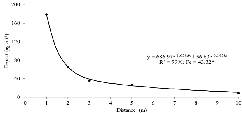
Figure 3. Curve fitting and regressions for tracer deposits at downwind distances in glyphosate + 2,4-D applications through AIXR 110015 nozzles.
