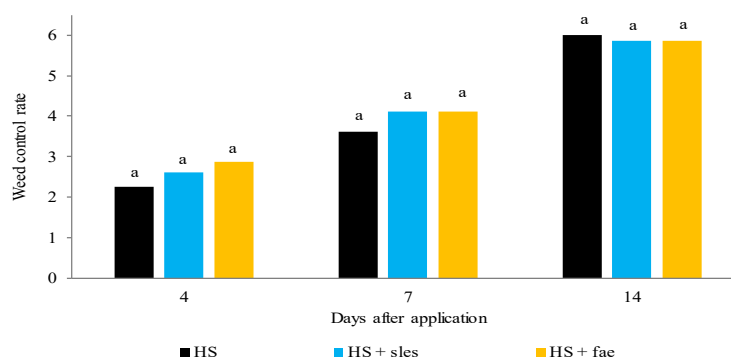
Figure 1. Effect of glyphosate + 2,4-D solutions on weed control at 4, 7 and 14 days after application through AIXR 11015 nozzles.
