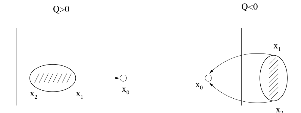
Figure 2: This figure shows the instanton effects in the p = 3 theory for real Q . When Q > 0 the cut (x_1, x_2) is in the real axis and the instanton is obtained by moving one brane from x_1 to x_0 . For Q < 0 , x_{1,2} are complex, with x_1 = x_2^* . The cut is parallel to the imaginary axis and there are two complex conjugate instantons obtained by moving the branes at the two edges of the cut.
