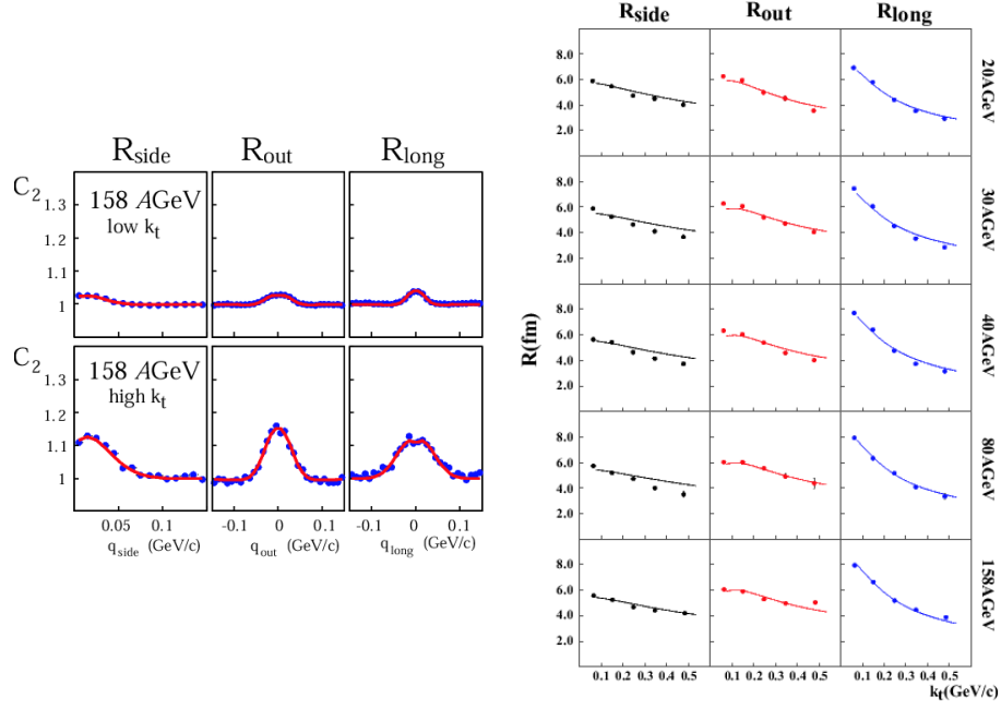
Fig. 3. Left: Projections of the \pi^- \pi^- correlation function on momentum difference q in the transverse (side, out) and beam (long) directions for central Pb+Pb collisions at 158 \text{ AGeV} . Right: Effective radius parameters R of the pion source versus mean transverse momentum k_t of the pion pairs in central Pb+Pb collisions at the five SPS energies. The curves show results of simultaneous fits of the blast wave model to the radius parameters and the transverse mass m_t spectra of pions and protons. All results refer to midrapidity pion pairs.
