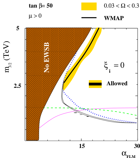
Figure 6: The same as in figure 2 but for \tan\beta = 50 .
