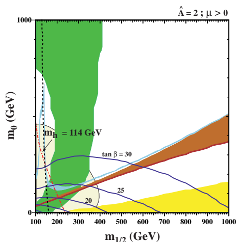
Fig. 8. The (m_{1/2}, m_0) plane in a mSUGRA scenario with the trilinear soft supersymmetry-breaking parameter \hat{A} = 2 . The green regions are excluded by b \rightarrow s\gamma , the brick-red regions because the LSP would be charged, and the yellow regions because of the cosmological light-element abundances [41].
