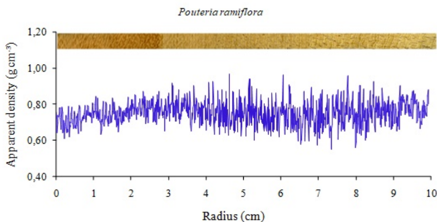
Figure 6. Radial profiles of the P. ramiflora wood apparent density.
