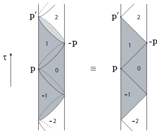
Figure 4: Poincaré patches of an arbitrary boundary point \mathbf{p} , separated by the null surfaces \mathbf{x} \cdot \mathbf{p} = 0 . Here AdS is represented as a cylinder with boundary \mathbb{R} \times S_{d-1} . Throughout this paper we shall mostly use a two-dimensional simplification of this picture, as shown in the figure. The point -\mathbf{p} and an image point \mathbf{p}' of \mathbf{p} are also shown.
