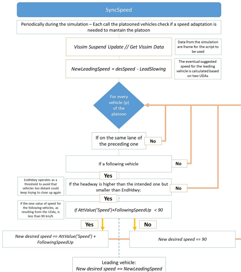
Figure 4. SyncSpeed function
