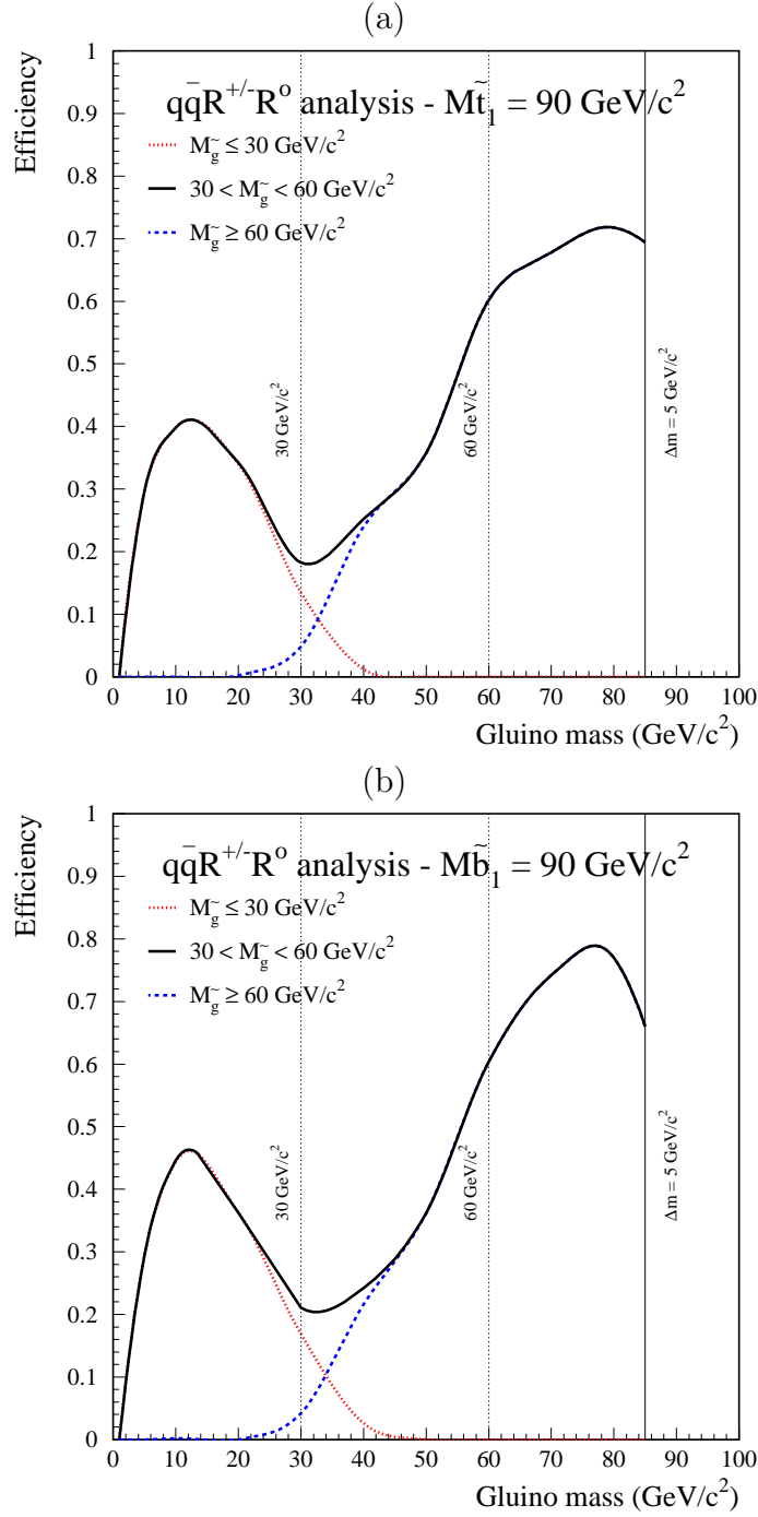
Figure 12: Signal detection efficiencies at \sqrt{s} = 200 \text{ GeV} for the stop (a) and sbottom (b) qqR^{\pm}R^0 analysis as a function of the gluino mass ( m_{\tilde{q}_1} = 90 \text{ GeV}/c^2 ). \Delta M is the mass difference between the squark and the gluino. Vertical lines show the limits of the mass analysis window. The last one ends at \Delta M = 5 \text{ GeV}/c^2 which corresponds the last simulated signal points.
