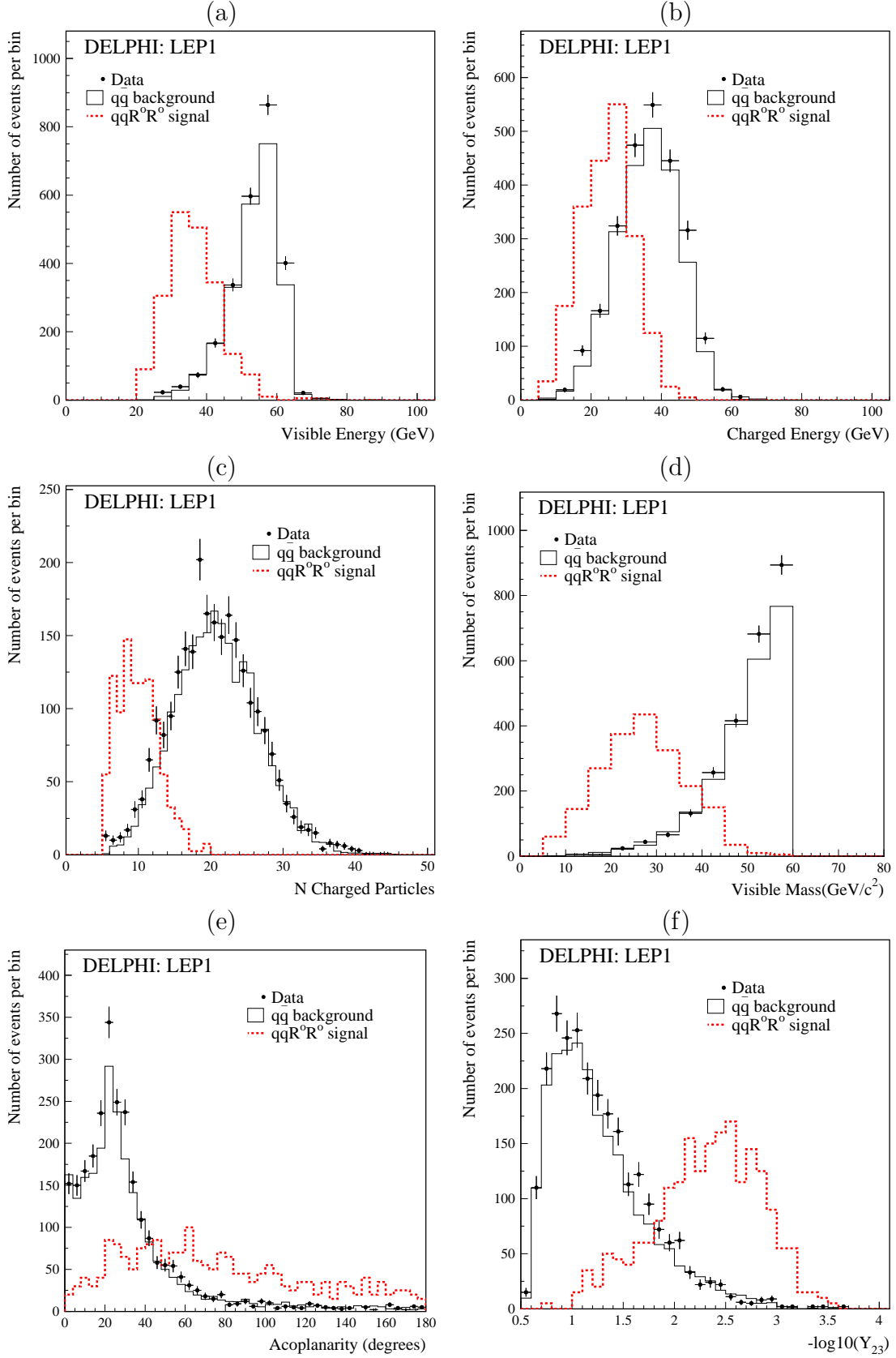
Figure 8: Comparison between data and simulation in the q\bar{q}R^0R^0 analysis at LEP1. (a) visible energy, (b) charged energy, (c) number of charged particles, (d) visible mass, (e) acoplanarity (f) DURHAM distance Y_{23} . Dotted lines show the q\bar{q}R^0R^0 signal distributions with arbitrary normalization when all simulated samples are added together.
