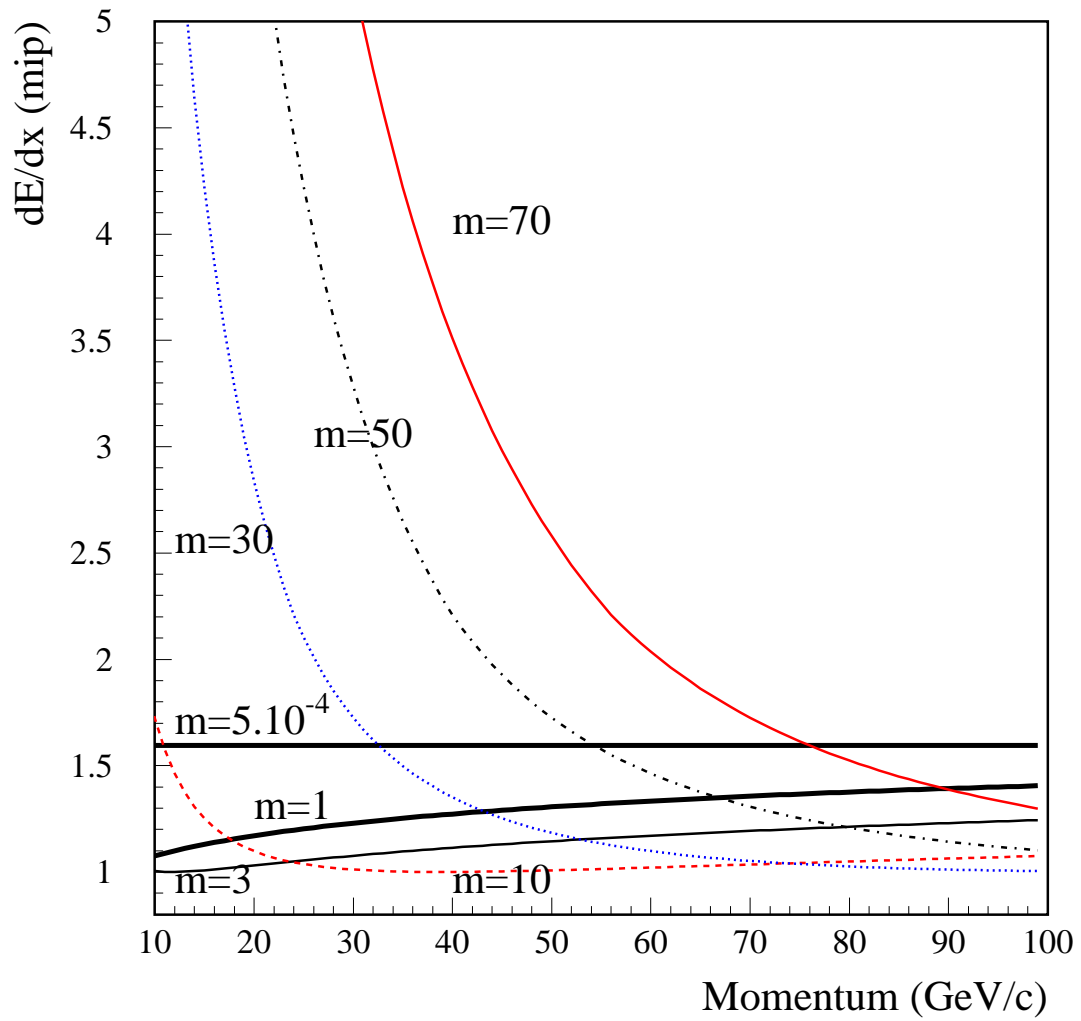
Figure 6: Ionization energy loss as a function of the momentum of the particle for different mass cases ( \text{GeV}/c^2 ). The dE/dx is expressed in units of energy loss for a minimum ionizing particle.
