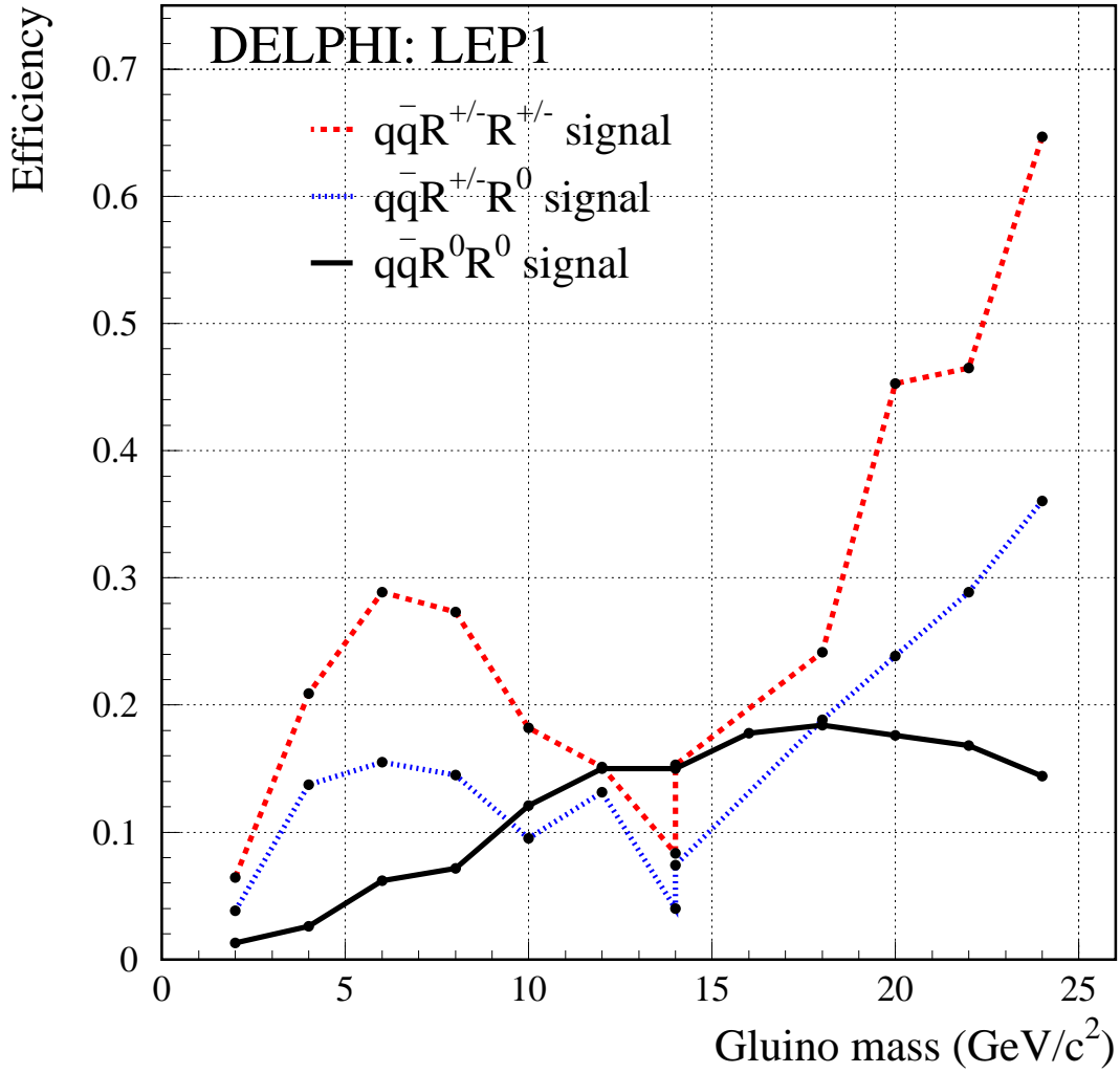
Figure 7: Signal detection efficiencies in the LEP1 data analysis as a function of the gluino mass for the three signal topologies q\bar{q}R^{\pm}R^{\pm} , q\bar{q}R^{\pm}R^0 and q\bar{q}R^0R^0 .
