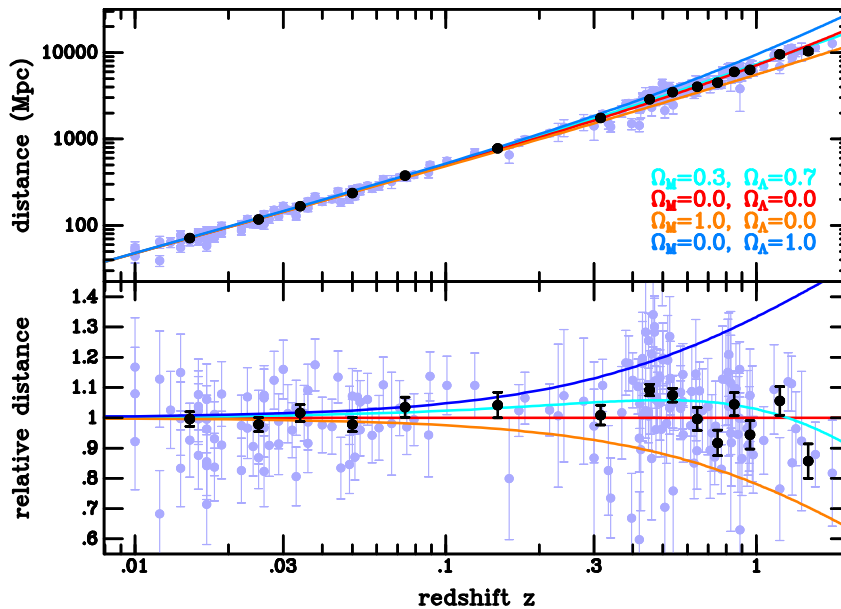
Figure 22: Type Ia supernovae Hubble diagram. The relative faintness of the distant supernovae relative to their nearby counterparts is apparent. A comparison with various cosmological models is made. Data from Riess et al. (2004).
