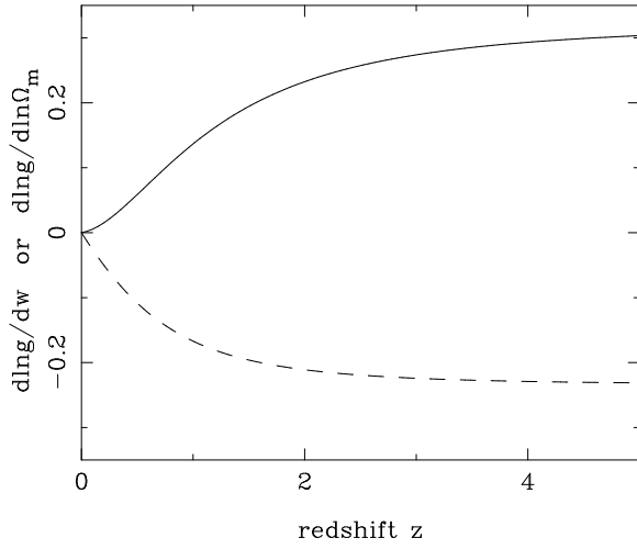
Figure 1: Perturbation of cosmological observables around a fiducial flat model with \Omega_m = 0.25 and w = -1 for the dark energy of the distance-redshift D(z) and growth factor-redshift g(z) relations. The solid line shows the effect of increase in w ; the dashed line the effect of an increase in \Omega_m .
