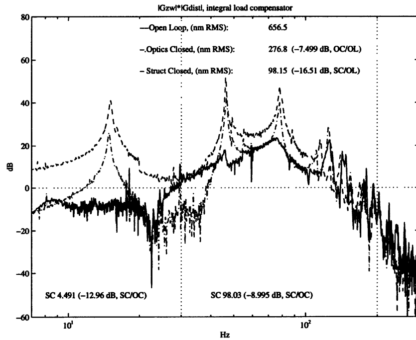
Figure C-16: Performance for the regular truss design, high frequency disturbances, high gain integral force feedback on midspan struts.
