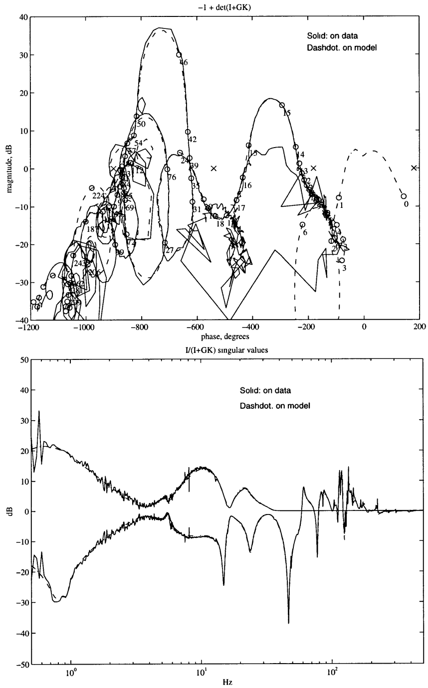
Figure 6-31: Multivariable Nichols plot and sensitivity singular values for regular configuration high frequency disturbances.
