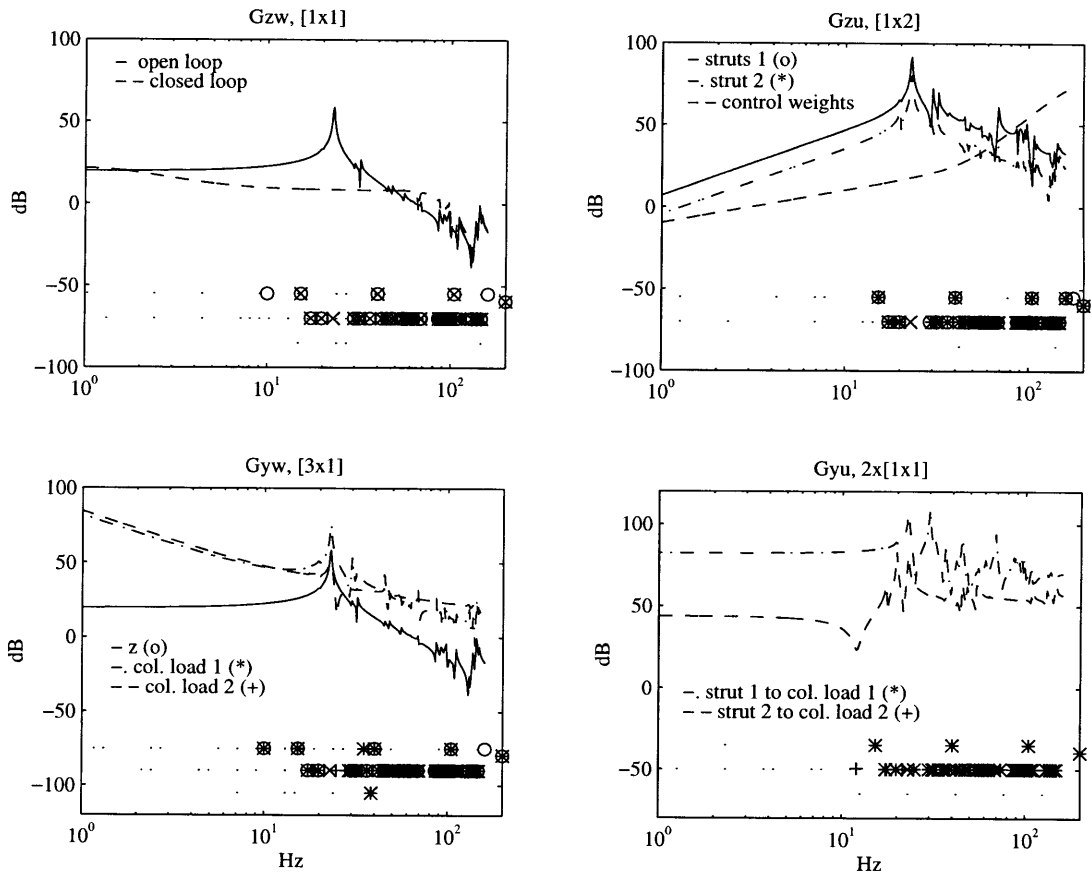
Figure 5-22: Condensed model block transfer functions for the best G.A. design. The closed loop rms performance is 33 nm with 75 N rms control effort.
