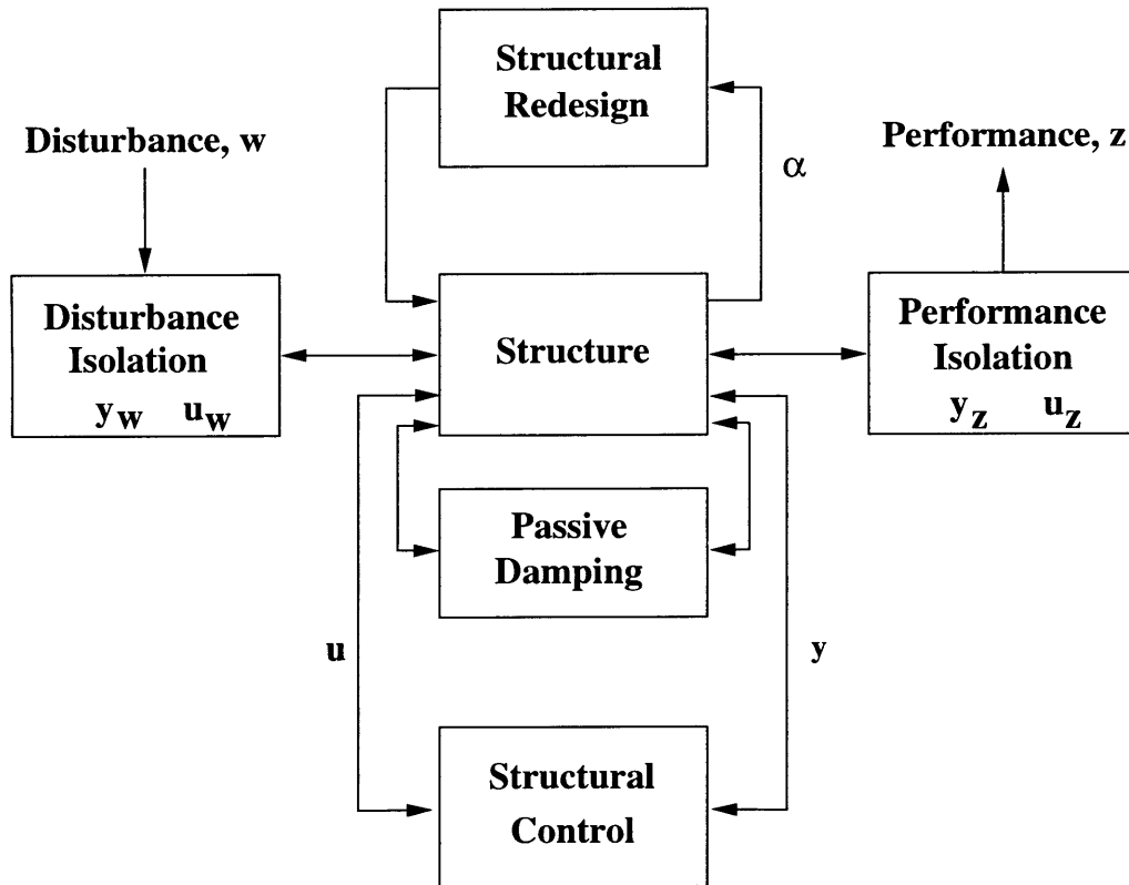
Figure 2-1: Overview of controls-structures design.
