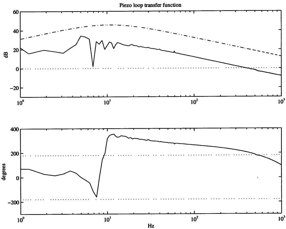
Figure B-2: Optical piezo loop transfer function, K_p G_p solid, controller, K_p dashed dot. The loop has moderate gain at low frequencies and is reduced at very low frequencies to avoid stack saturation due to laser drift.
