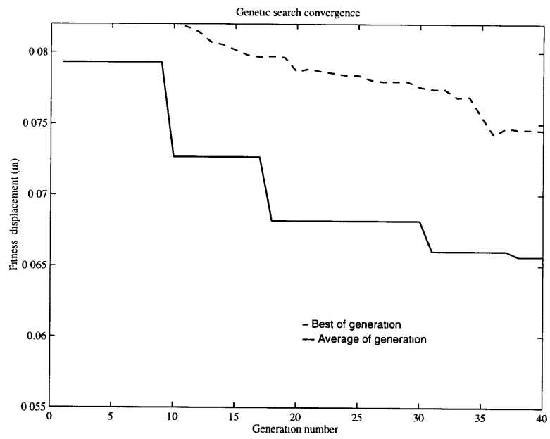
Figure 4-10: Displacement minimization genetic convergence for two trials
