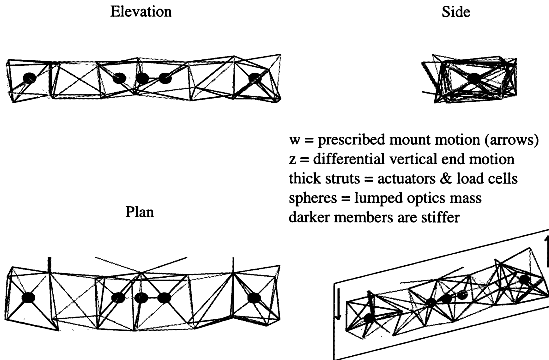
Figure 5-21: Four view of the optimized box truss structure.
