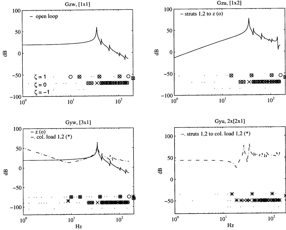
Figure 5-20: Nominal full system block transfer functions.
