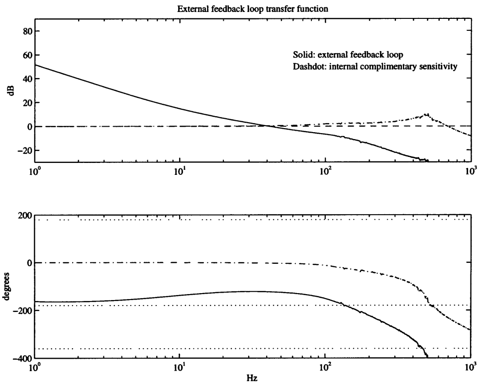
Figure B-7: External loop transfer function, C_{odl}K_f solid, where C_{odl} is the complimentary sensitivity of the closed internal loop. This shows why the actuators are ganged in the internal loop in order to track the external fringe.
