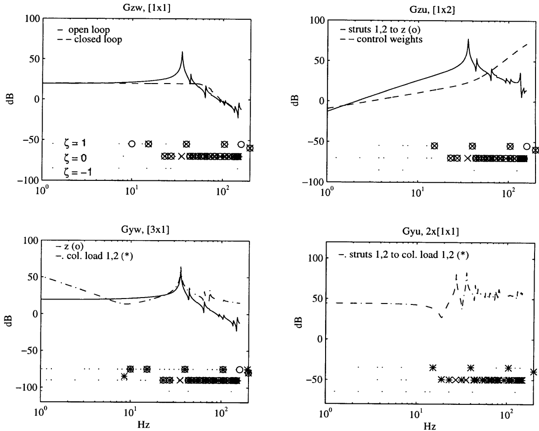
Figure 5-19: Nominal condensed system block transfer functions. The closed loop rms performance is 110 nm with 68 N rms control effort.
