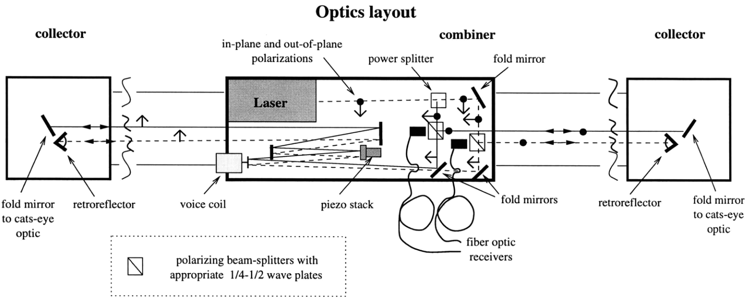
Figure 6-5: Plan view of the optical layout with arrows and dots representing in and out-of-plane polarizations
