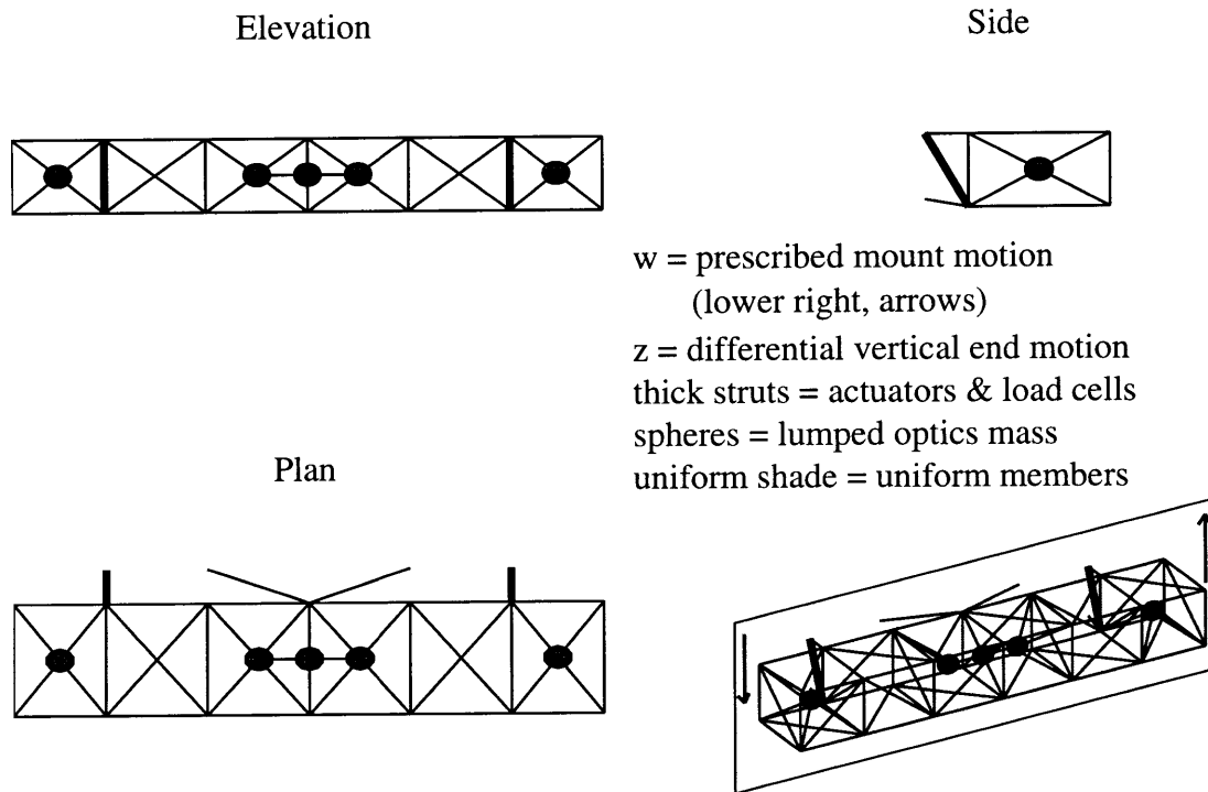
Figure 5-17: Four view of the nominal box truss structure.
