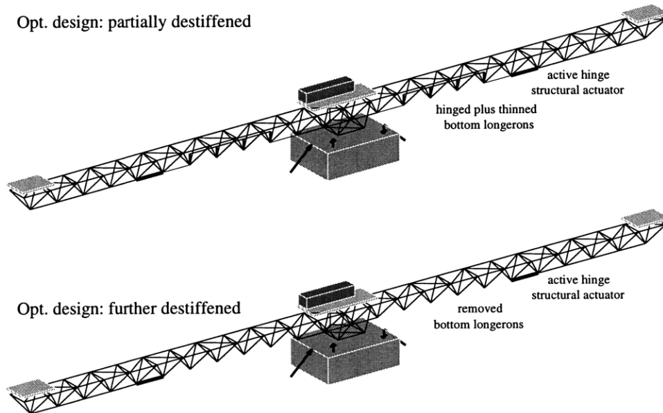
Figure 6-34: Genetic Algorithm partially flexible configurations for high frequency disturbances.
