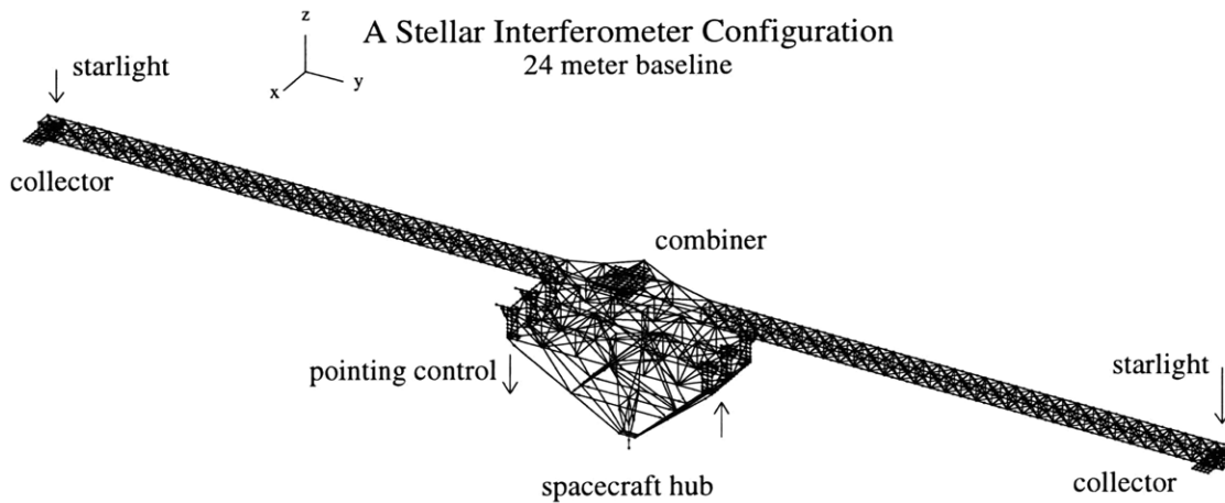
Figure 5-1: Line drawing of an interferometric spacecraft
