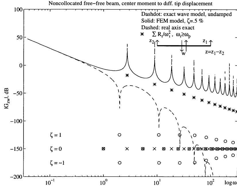
Figure 2-7: Beam noncollocated transfer function magnitude where a 52 element FEM is compared to the exact solution.
