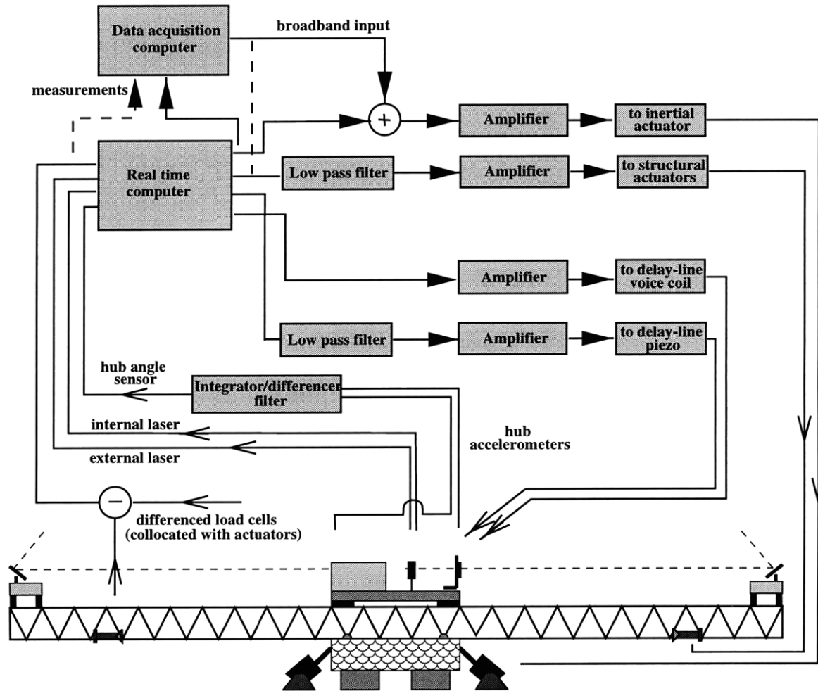
Figure 6-8: System schematic showing origination and destination of measurement and control signals. Note that data is primarily taken through the real time computer incorporating sampling delay in the measurements.
