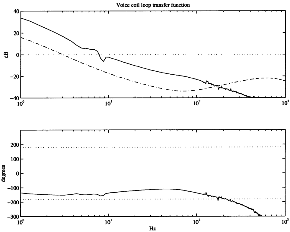
Figure B-4: Optical voice coil loop transfer function, K_v G_v solid, controller, K_v dashed dot. The loop has high gain at low frequencies to desaturate the piezo when used as a servo.
